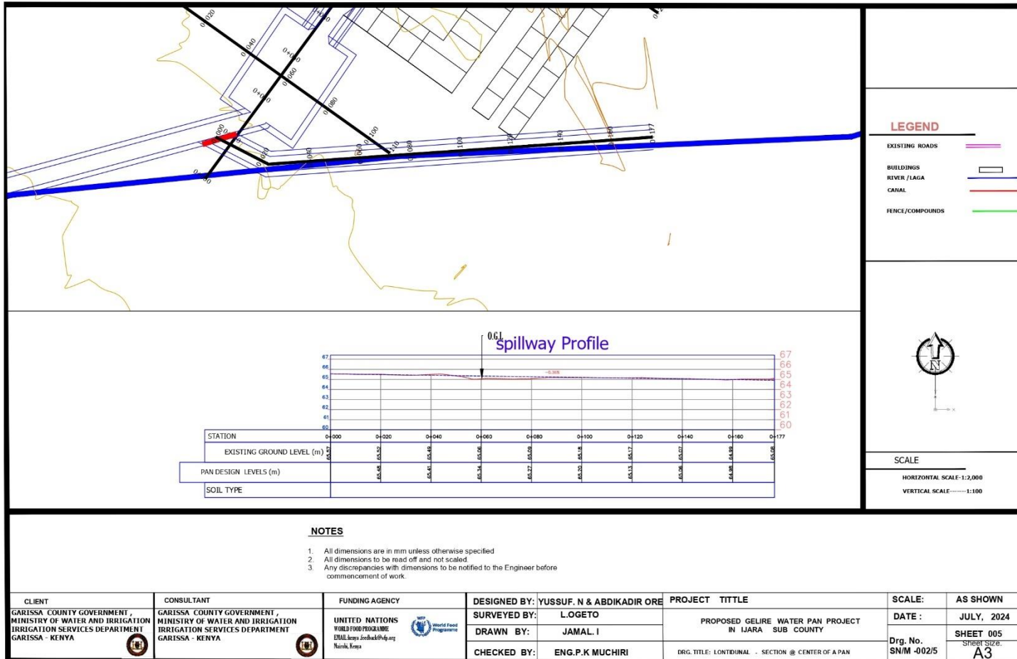
Figure 8 Spillway profile
