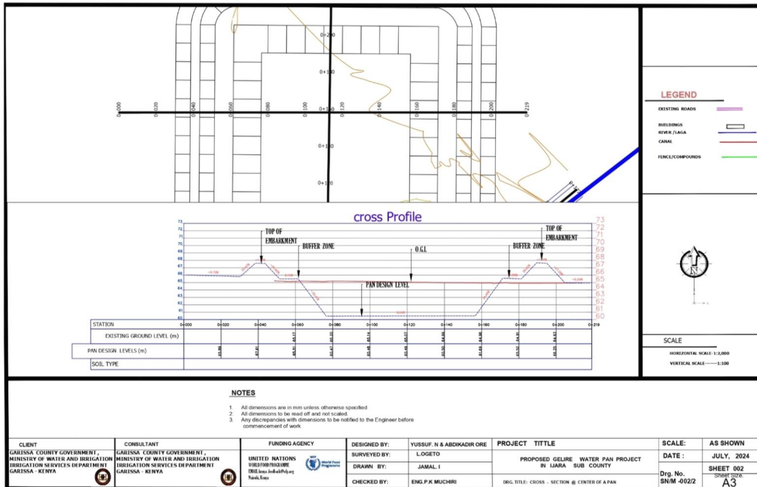
Figure 2 Cross-section profile
