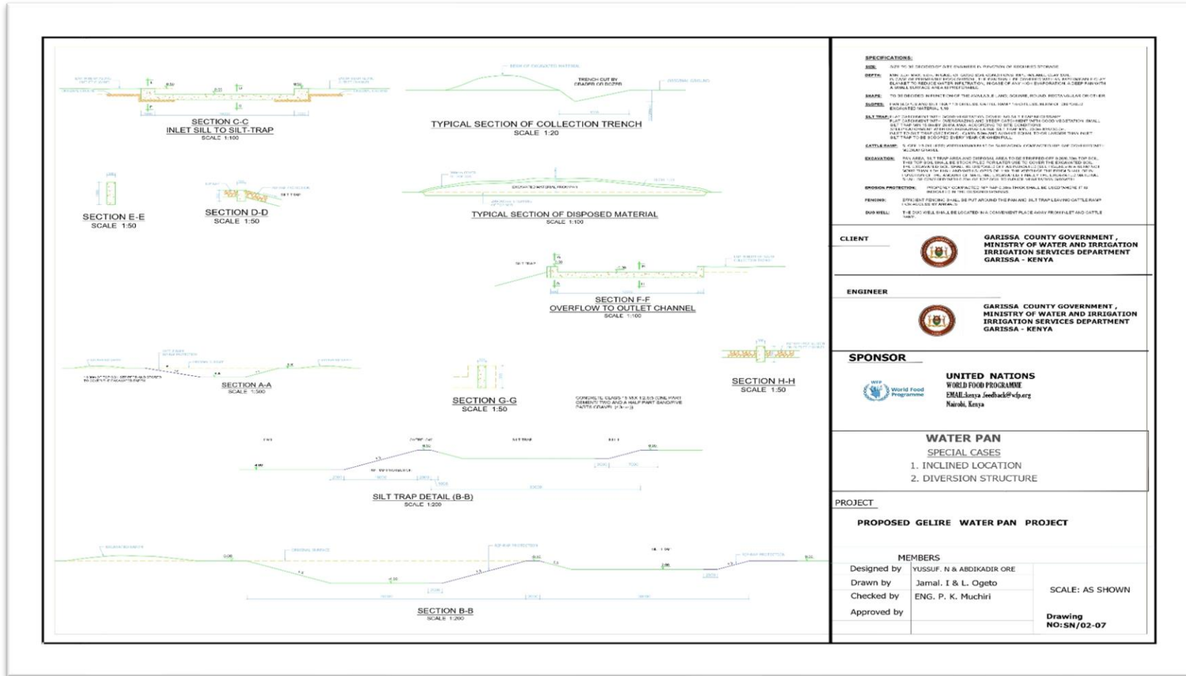
Figure 1 Water pan special cases
