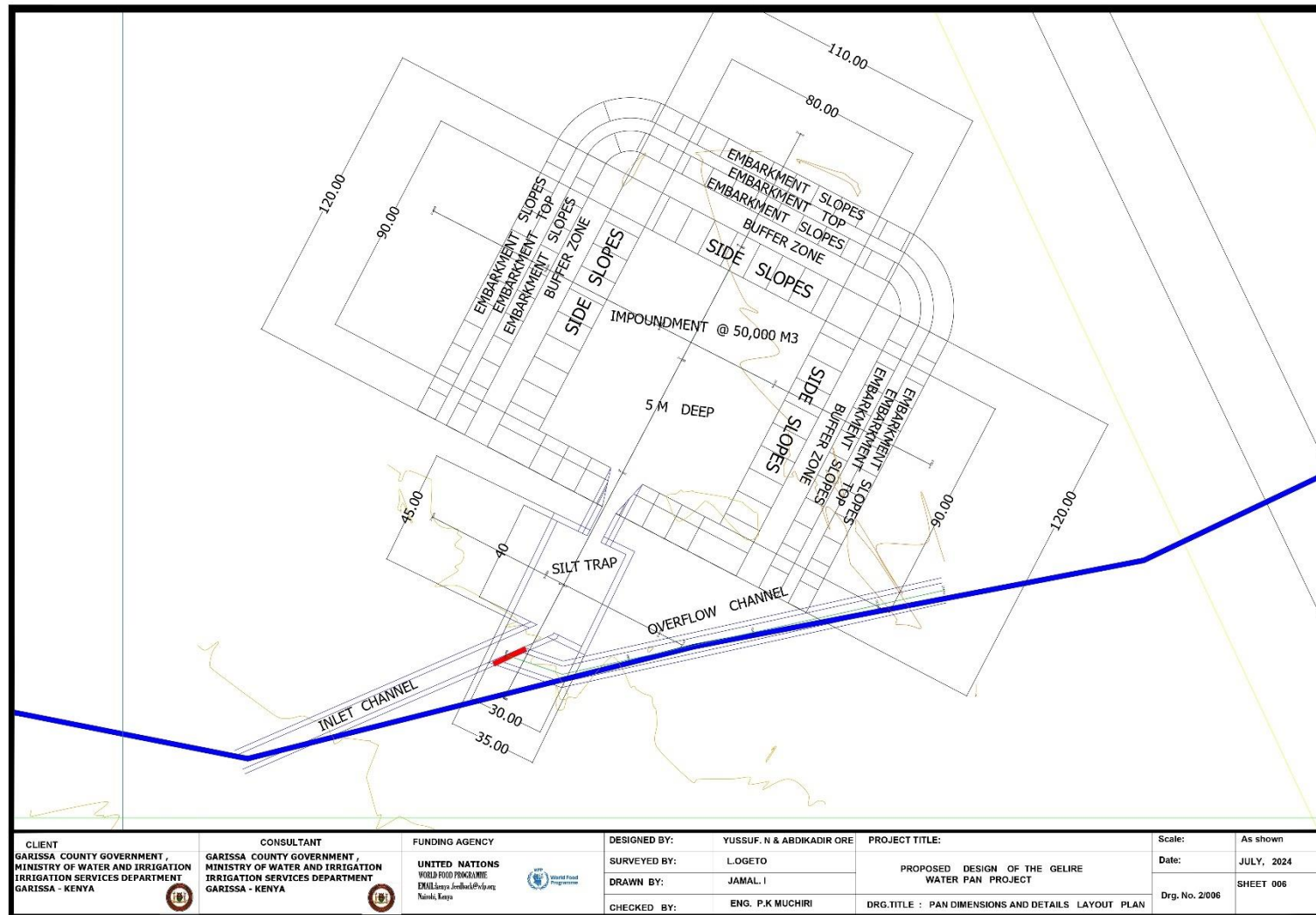
Figure 4 Dimension layout
