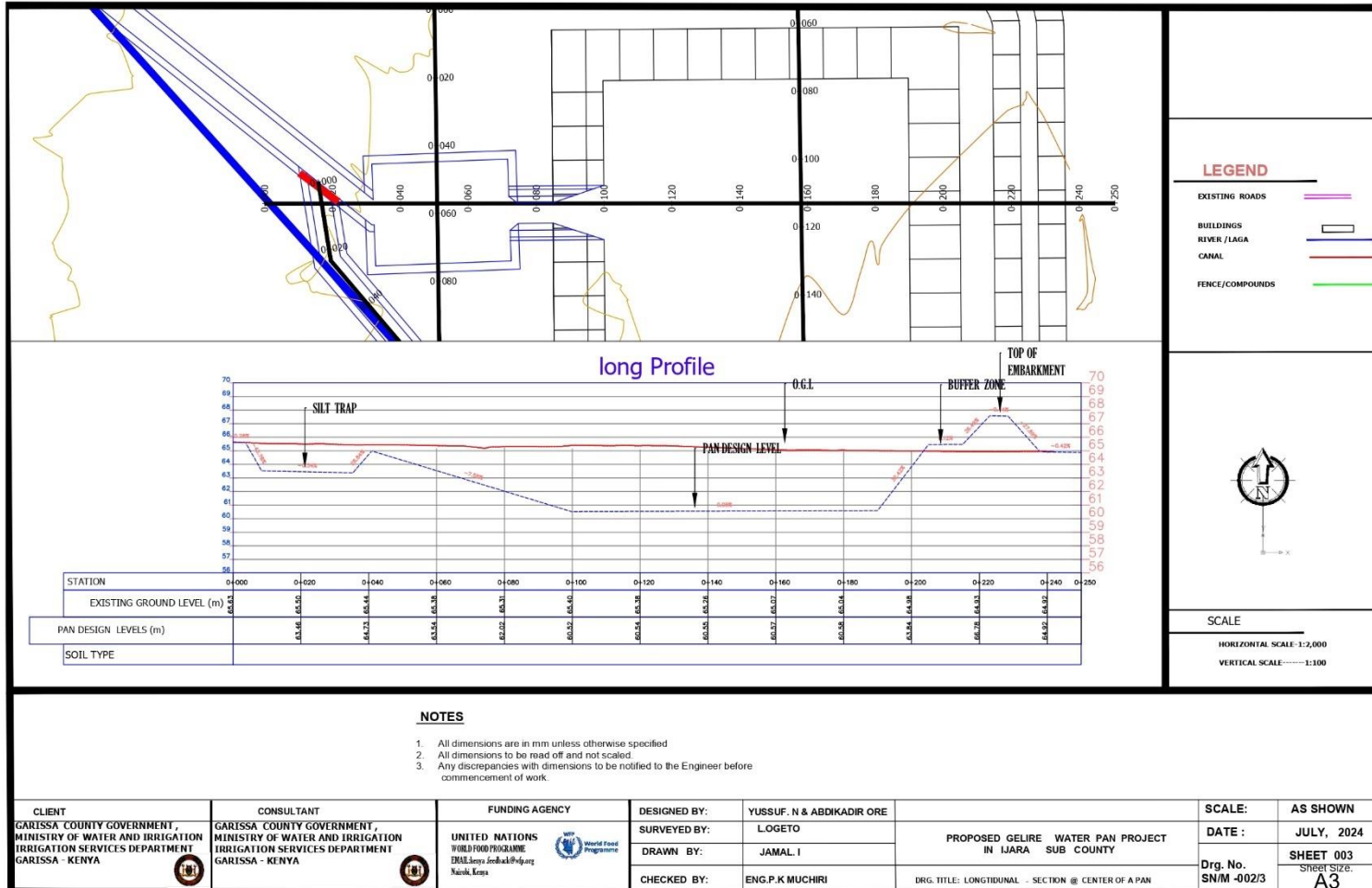
Figure 5 Longitudinal profile
