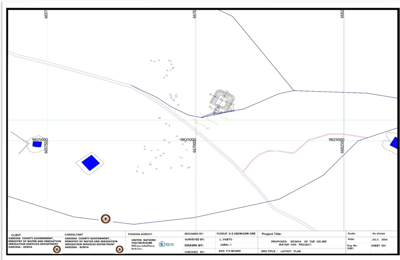
Figure 3 Water pan layout
