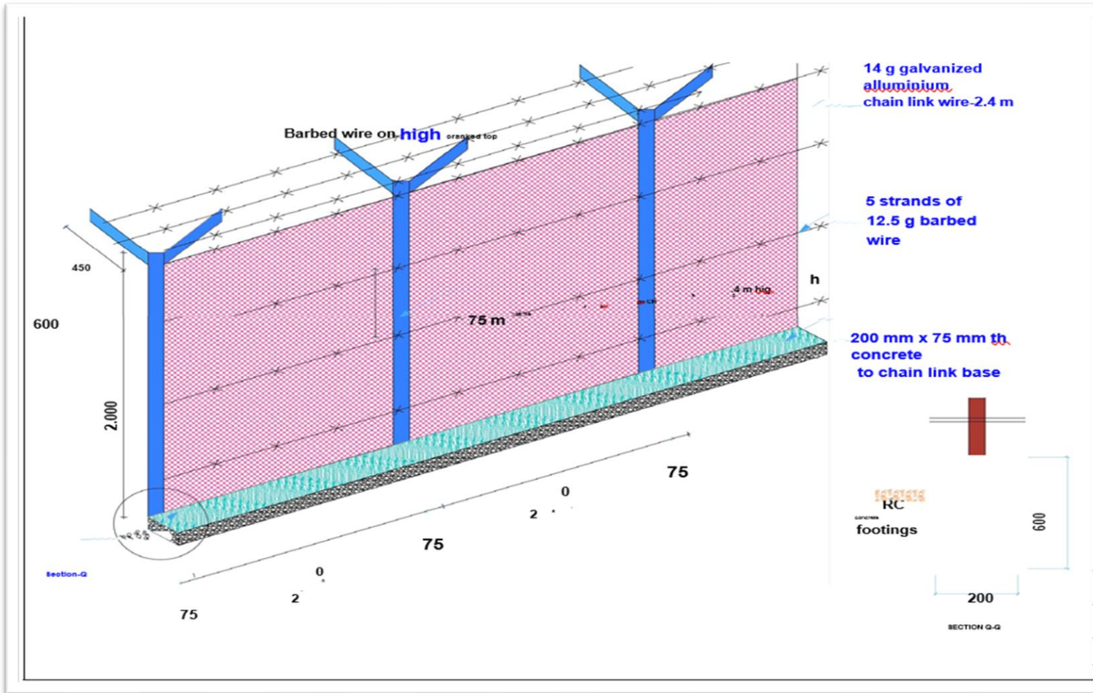
Figure 14 Details of fencing
