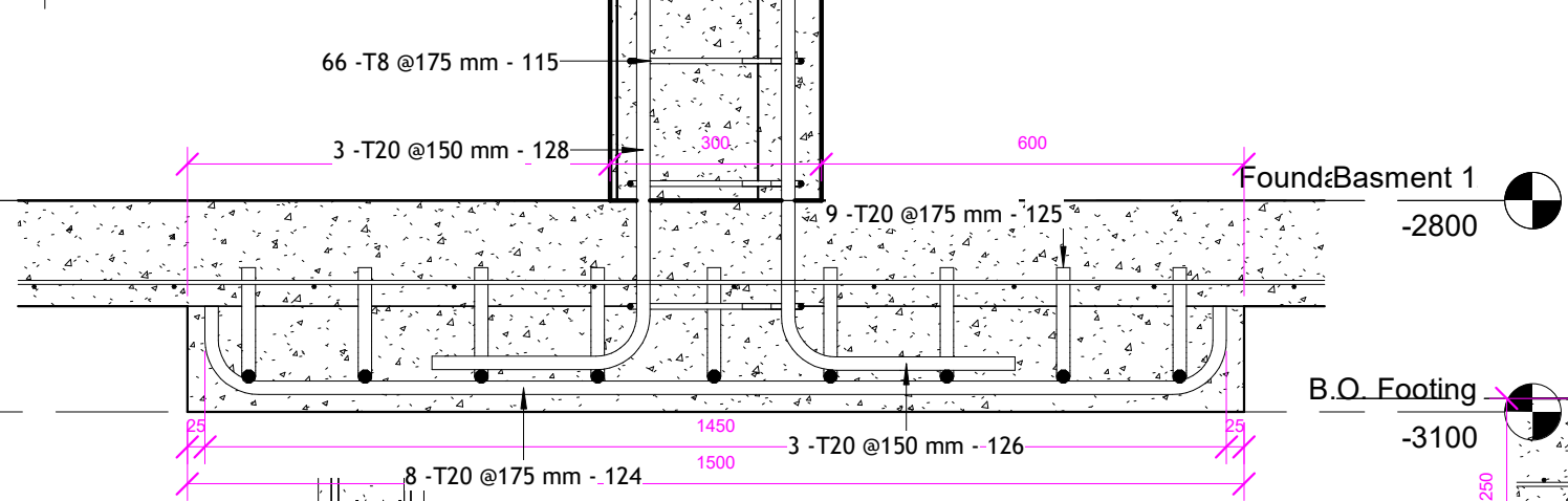
13 Column base b1 section 1 : 10
