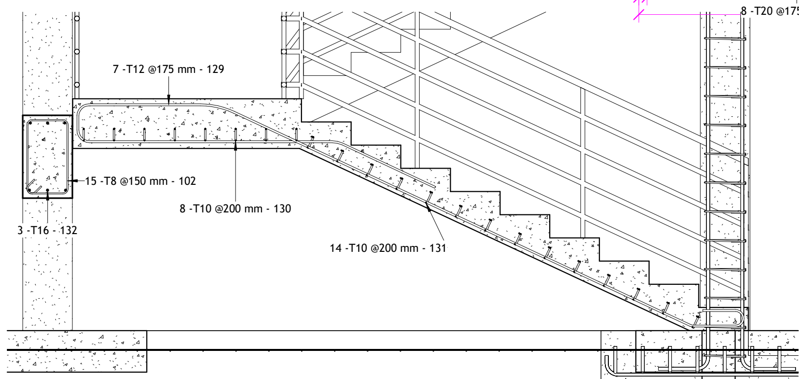
16 Staircase section 1 : 20
