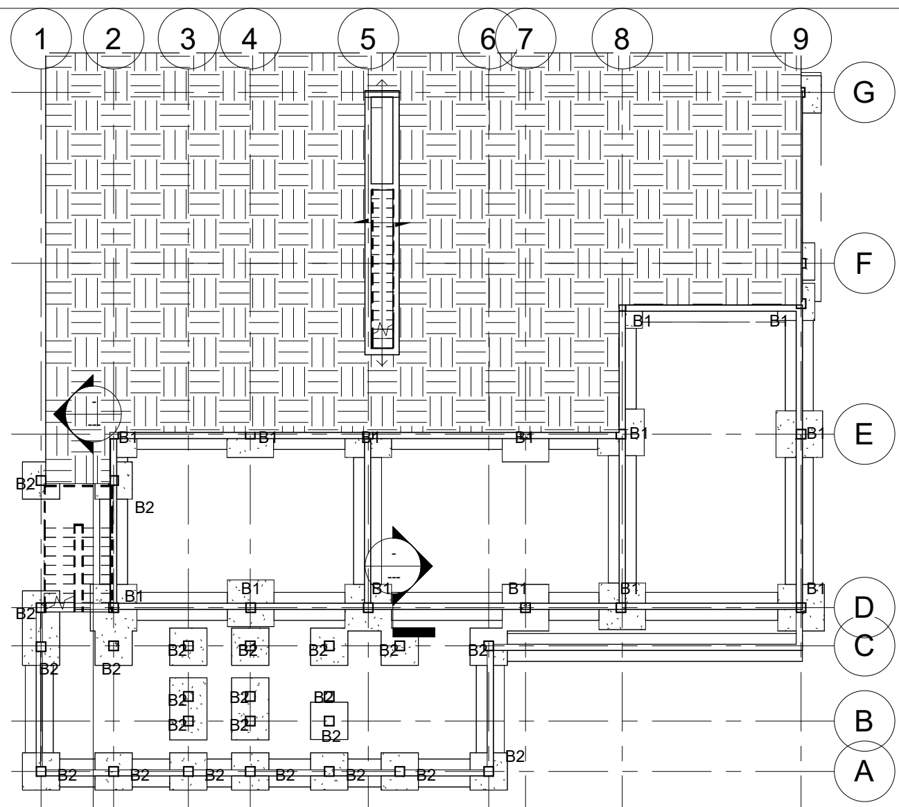
1 Foundation layout 1 : 150
