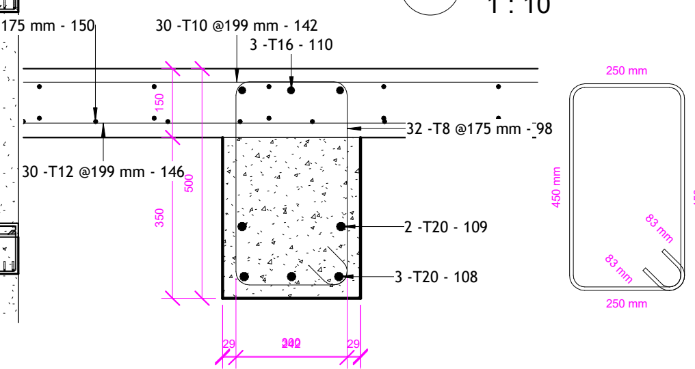
12 Beam B4 Section 1 : 10
