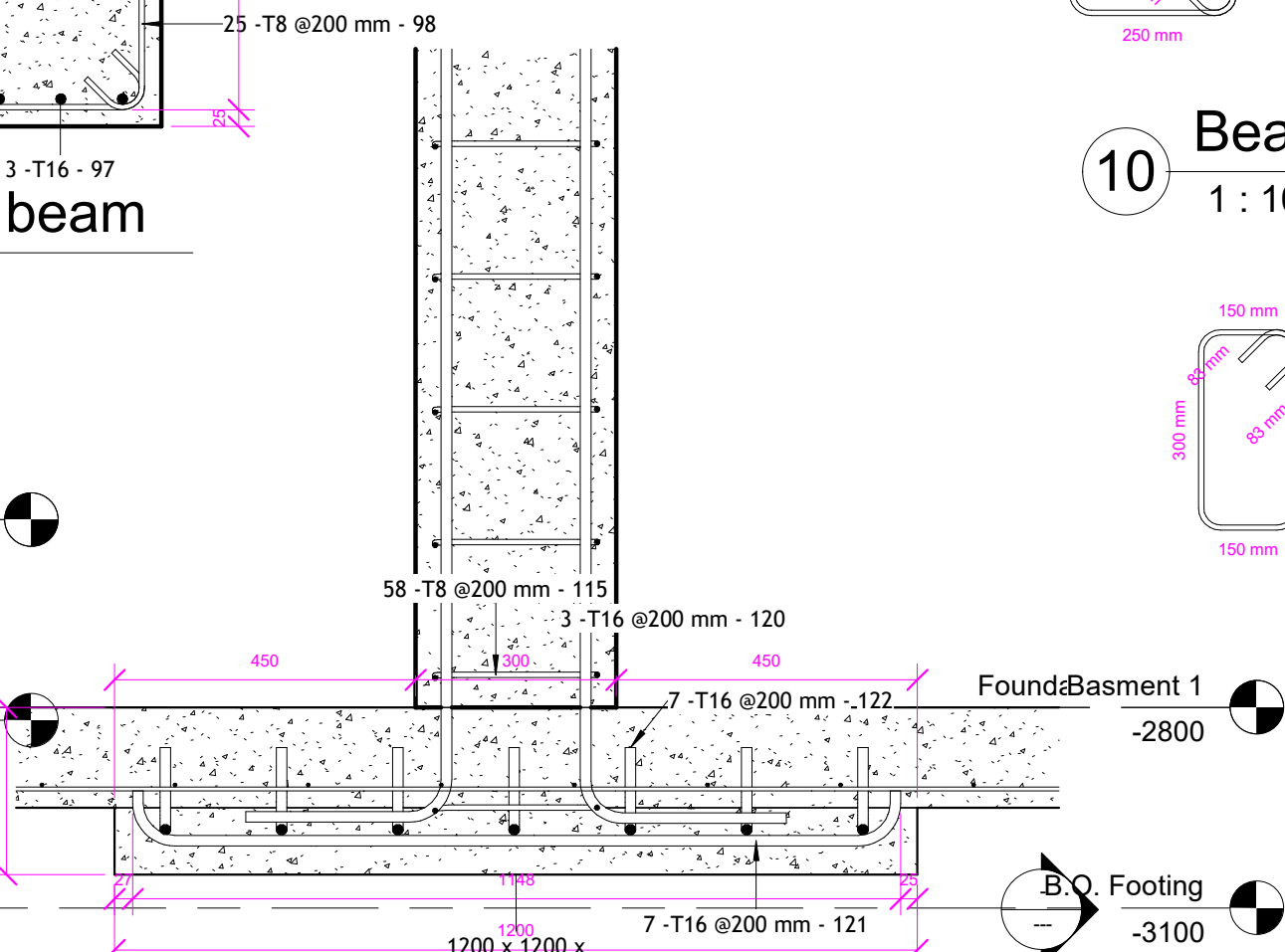
14 Column base b2 section 1 : 10
