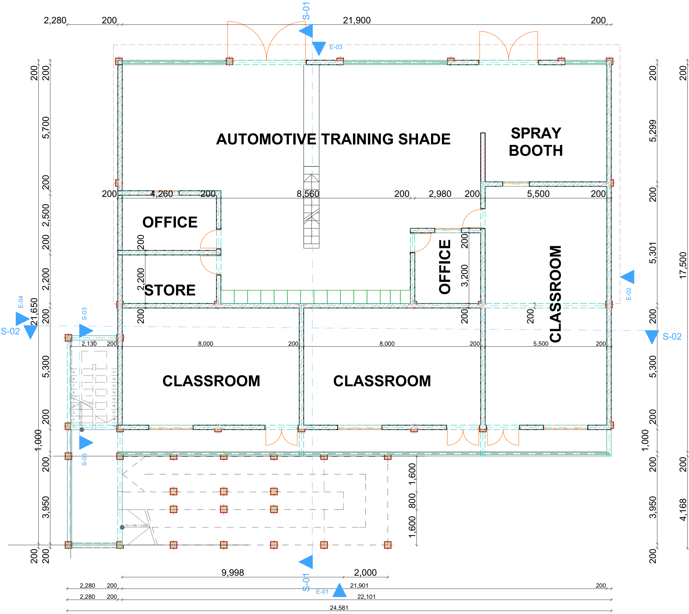
GROUND FLOOR LAYOUT PLAN
