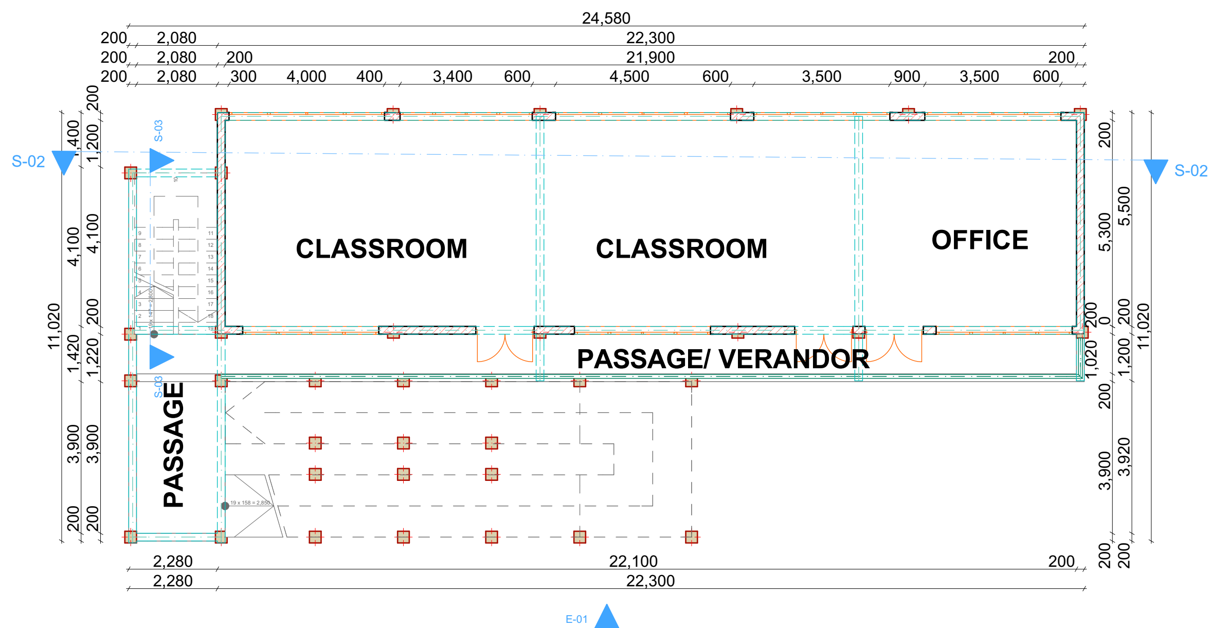
FIRST FLOOR LAYOUT
