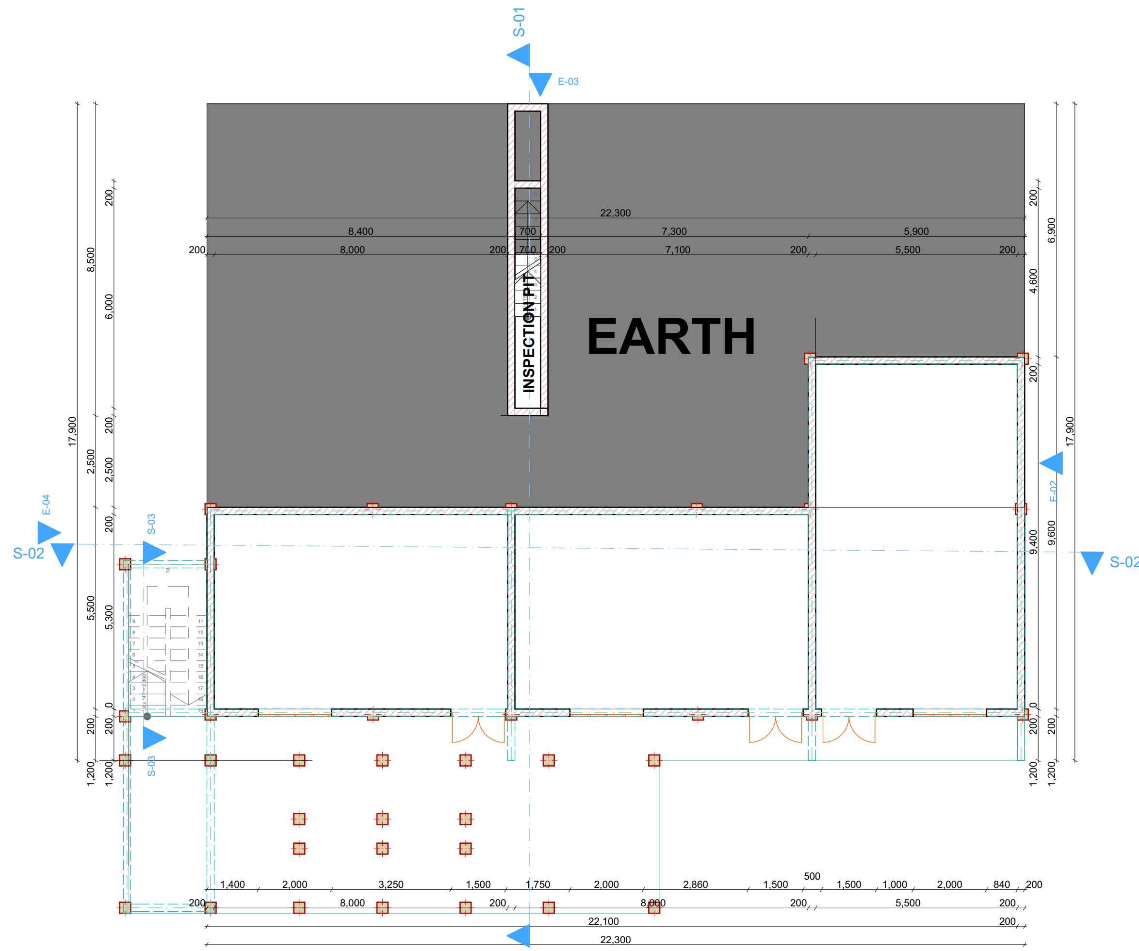
BASEMENT FLOOR
