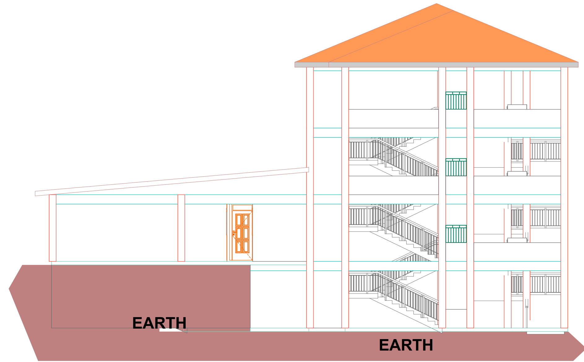
ELEVATION E-04
