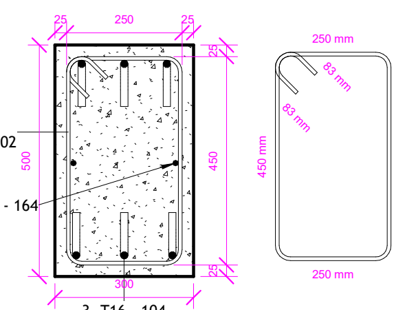
9 Beam B1 Section 1 : 10
