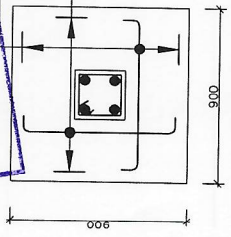
300x300MM COLUMN STUB C1 ON 900x900x300 TYPICAL BASE B1 SCALE 1:25
