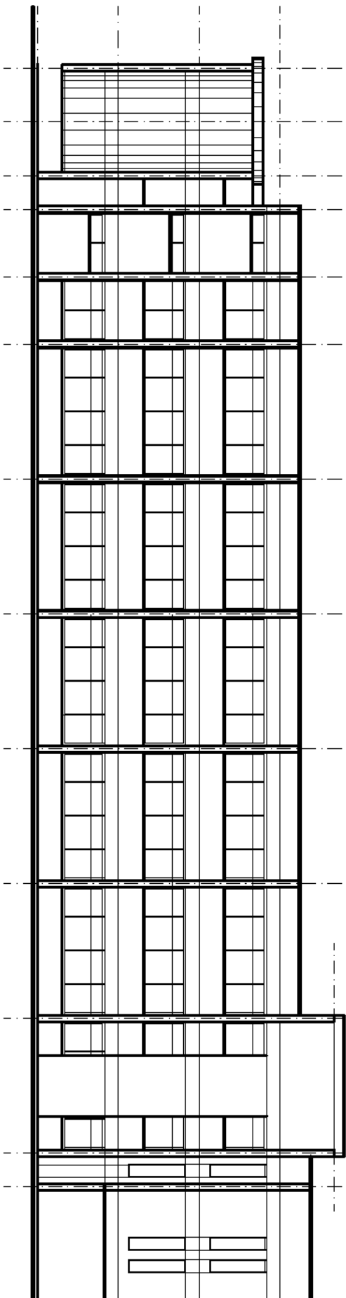
LEFT ELEVATION
