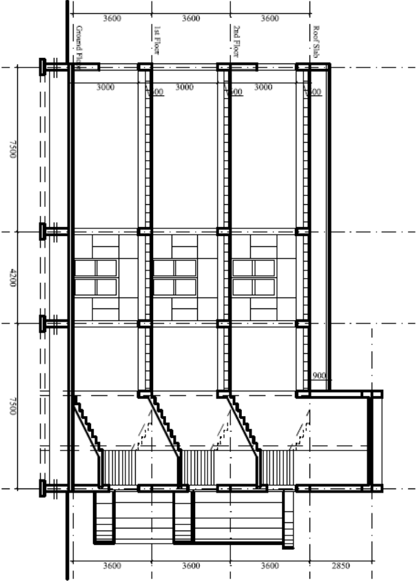
SECTION ELEVATION
