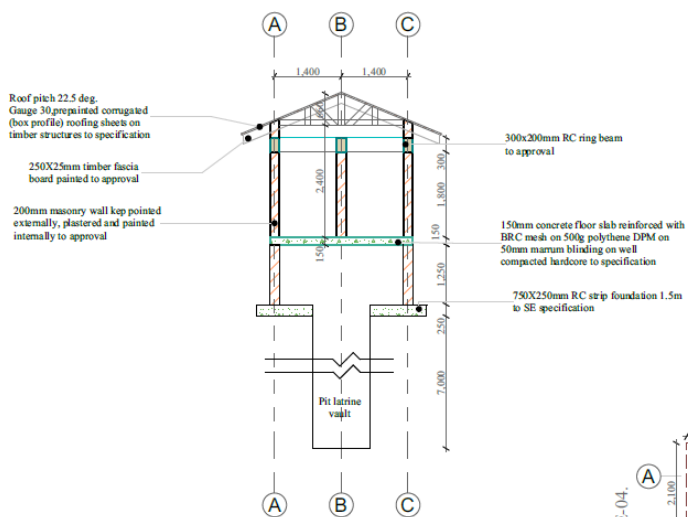
SECTION 01 SCALE 1:100
