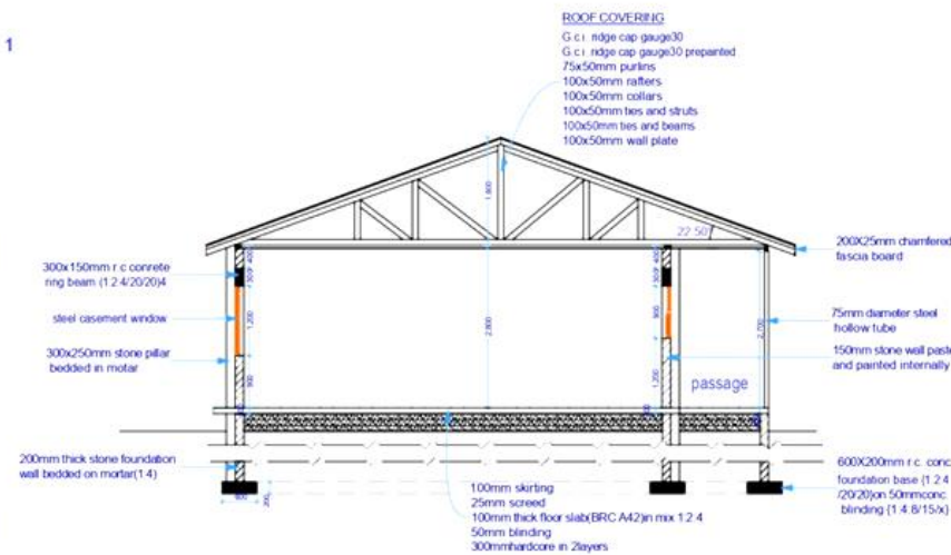
SECTION 01-01
