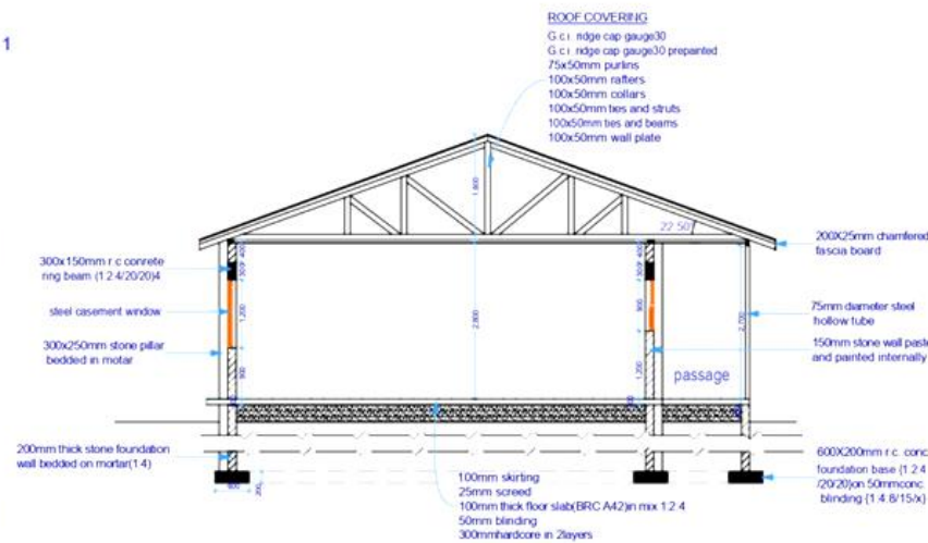
SECTION 01-01
