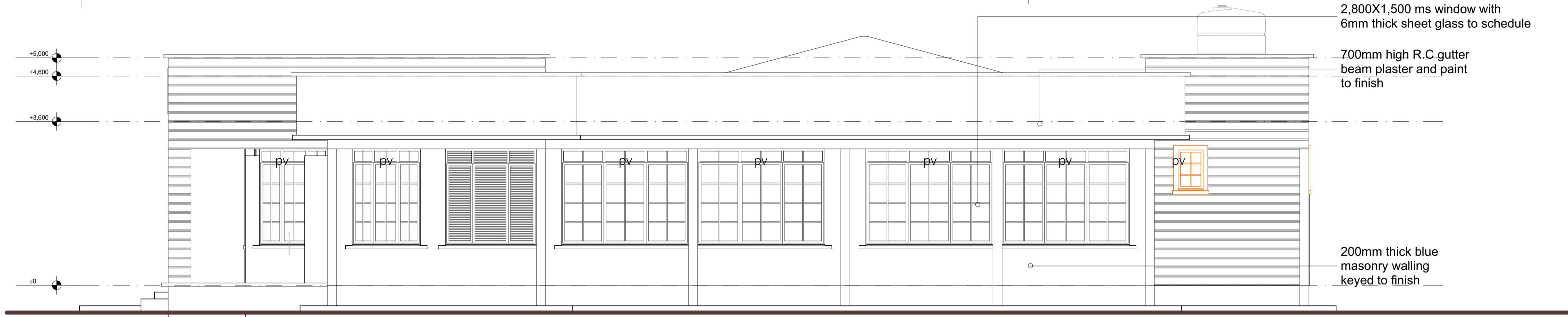
ELEVATION E-2 SCALE 1:100
