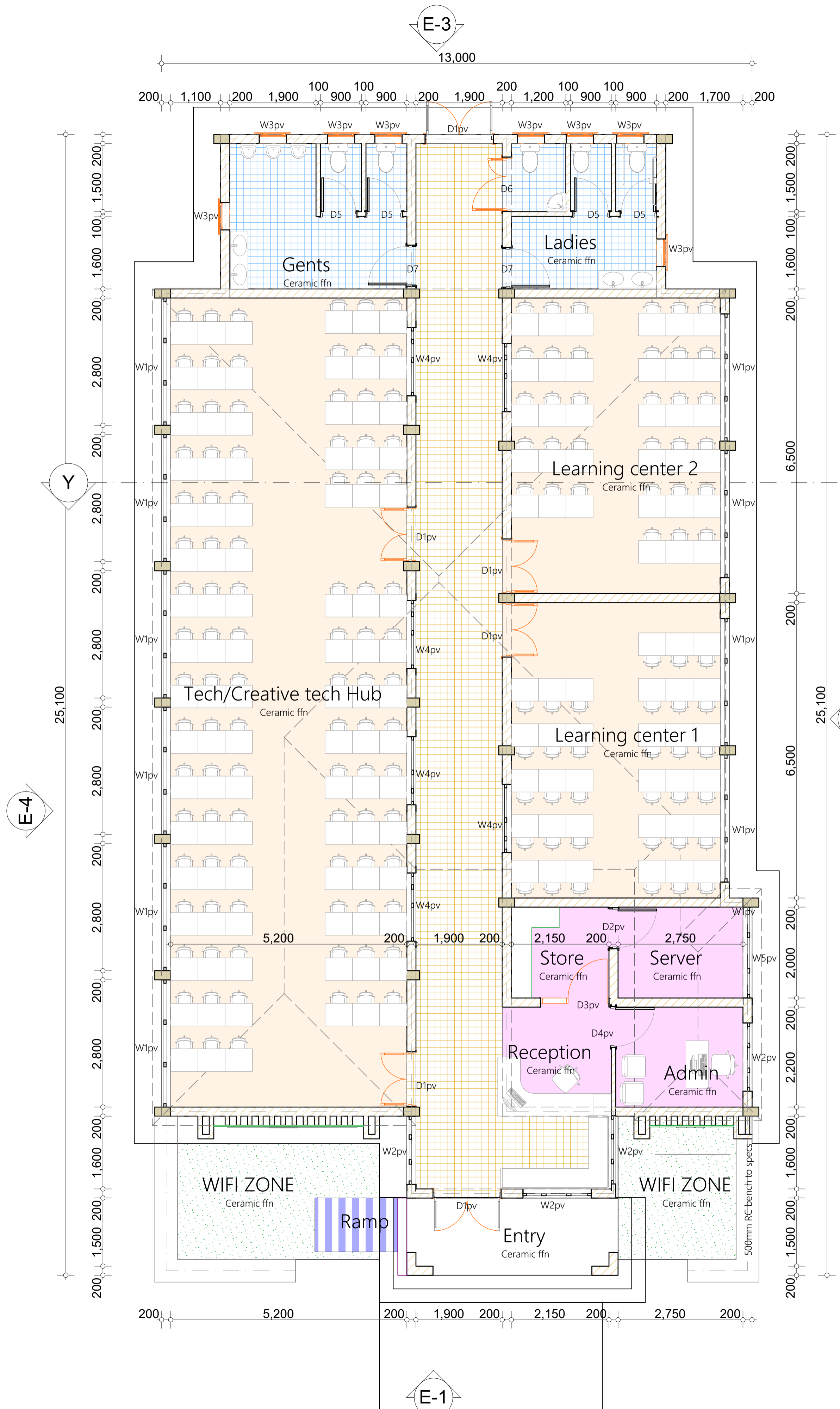
FLOOR LAYOUT PLAN SCALE 1:100
