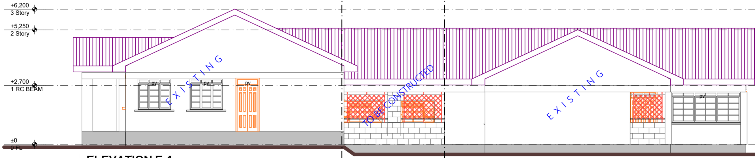
ELEVATION E-4 scale 1:100
