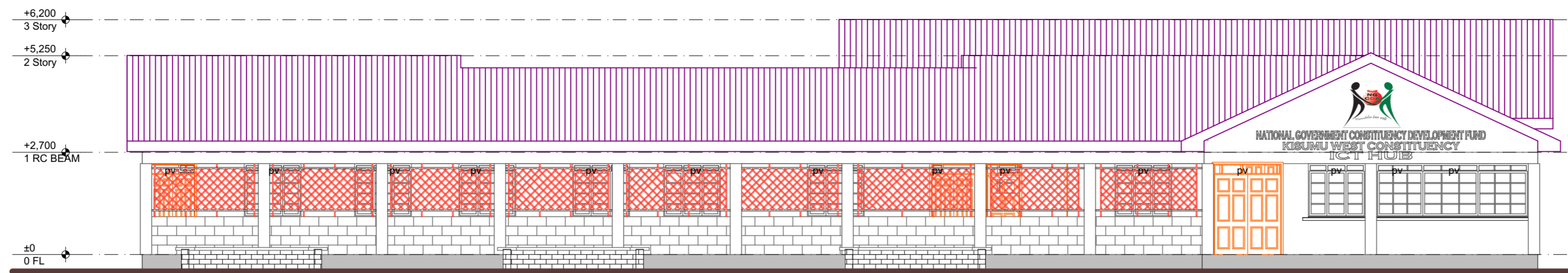
ELEVATION E-1 scale 1:100
