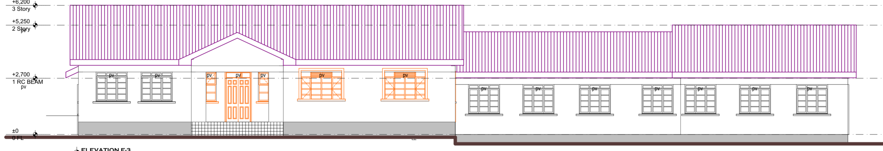
ELEVATION E-3 scale 1:100
