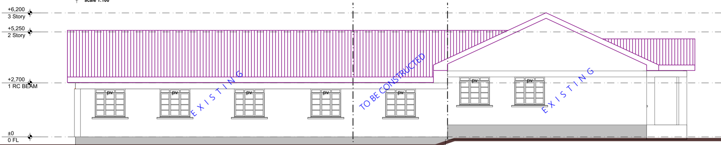
ELEVATION E-2 scale 1:100
