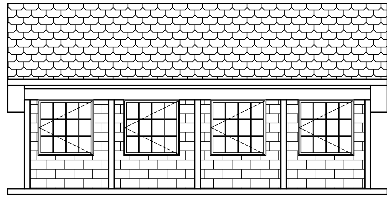
NORTH ELEVATION
