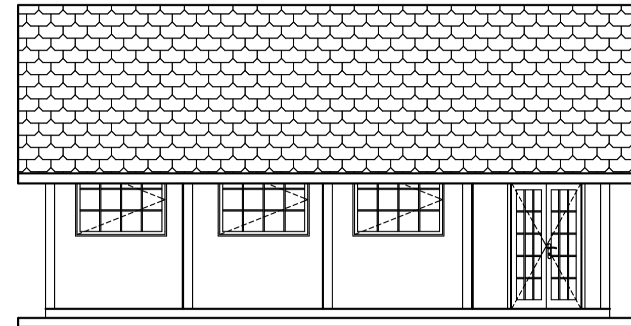
SOUTH ELEVATION
