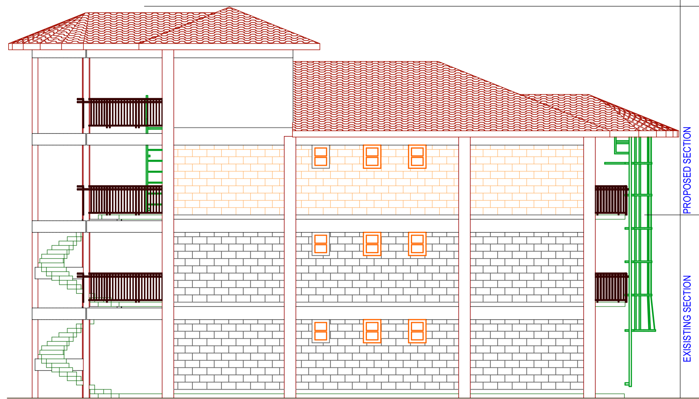
ELEVATION 03
