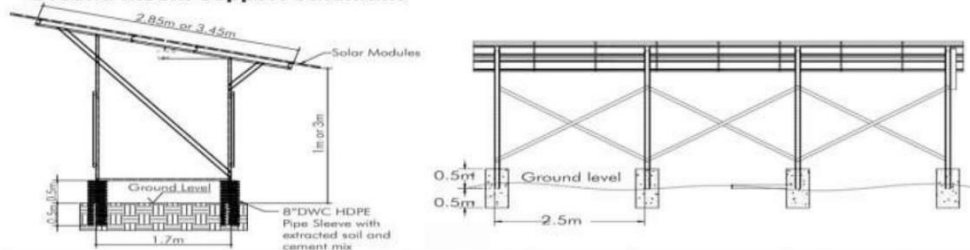
Ground Mount Support Schematic
