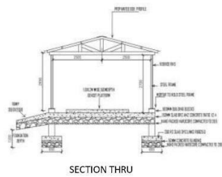
SECTION THRU
