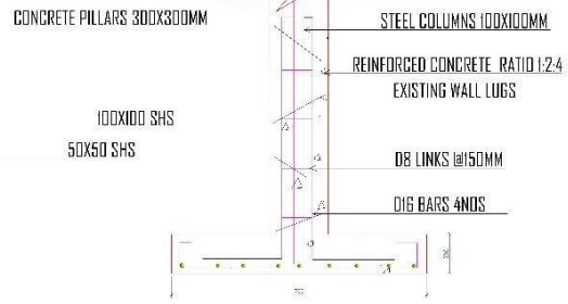
COLUMN FOUNDATION SECTION
