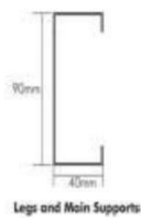
Legs and Main Supports
