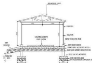
SECTION THRU
