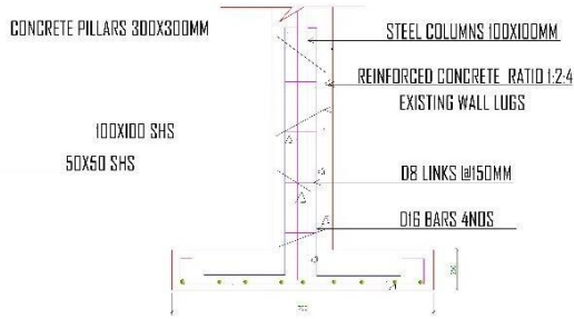
COLUMNS FOUNDATION SECTION
