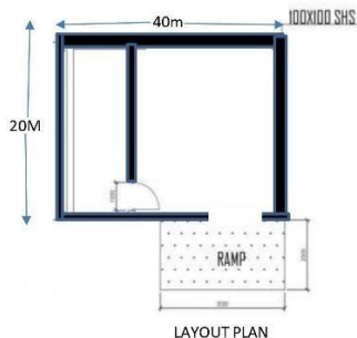
LAYOUT PLAN
