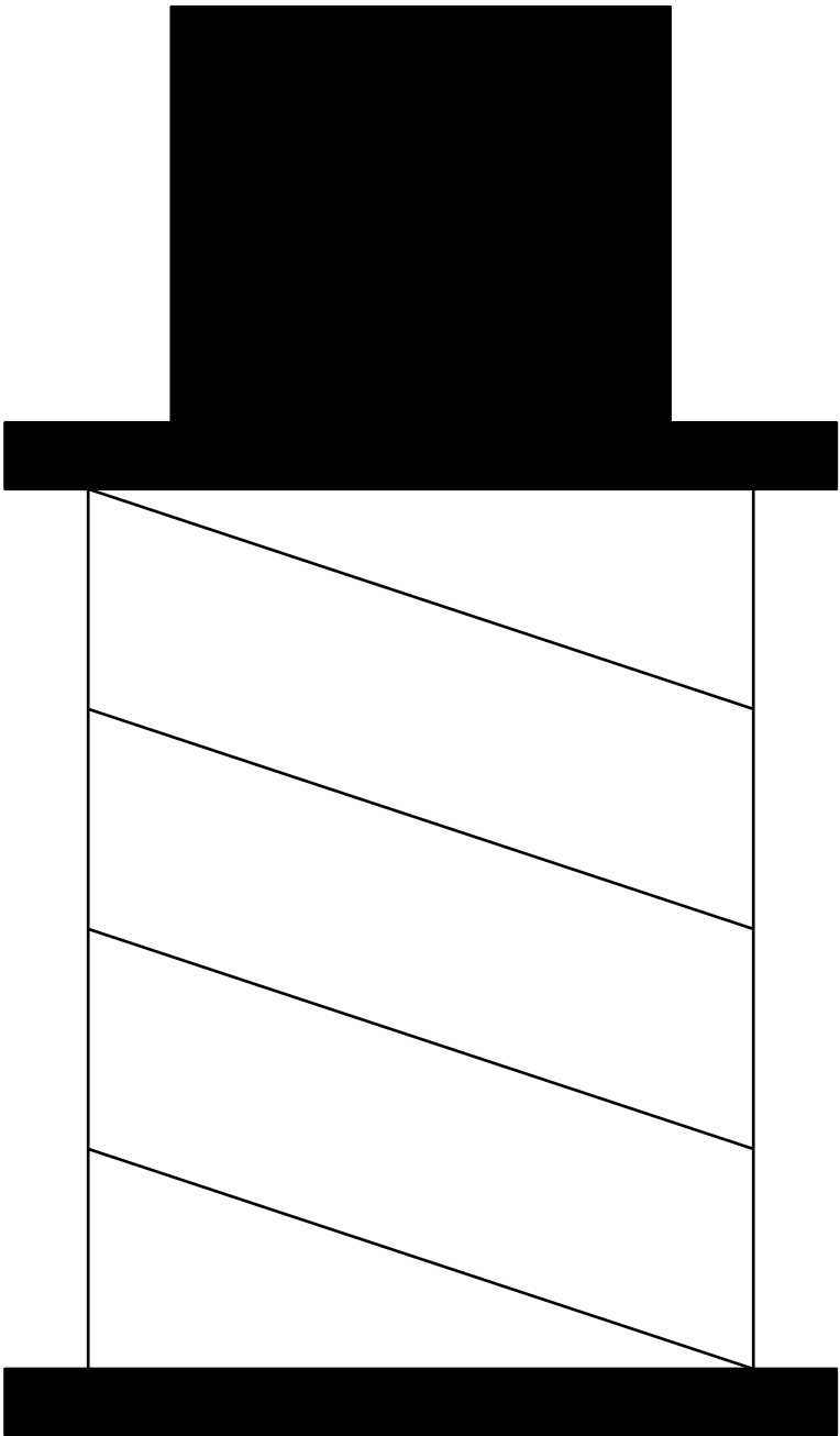
RC Pad Foundation 1200x1200x600mm
