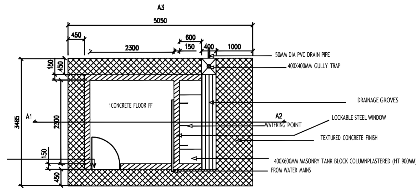
LAYOUT PLAN
