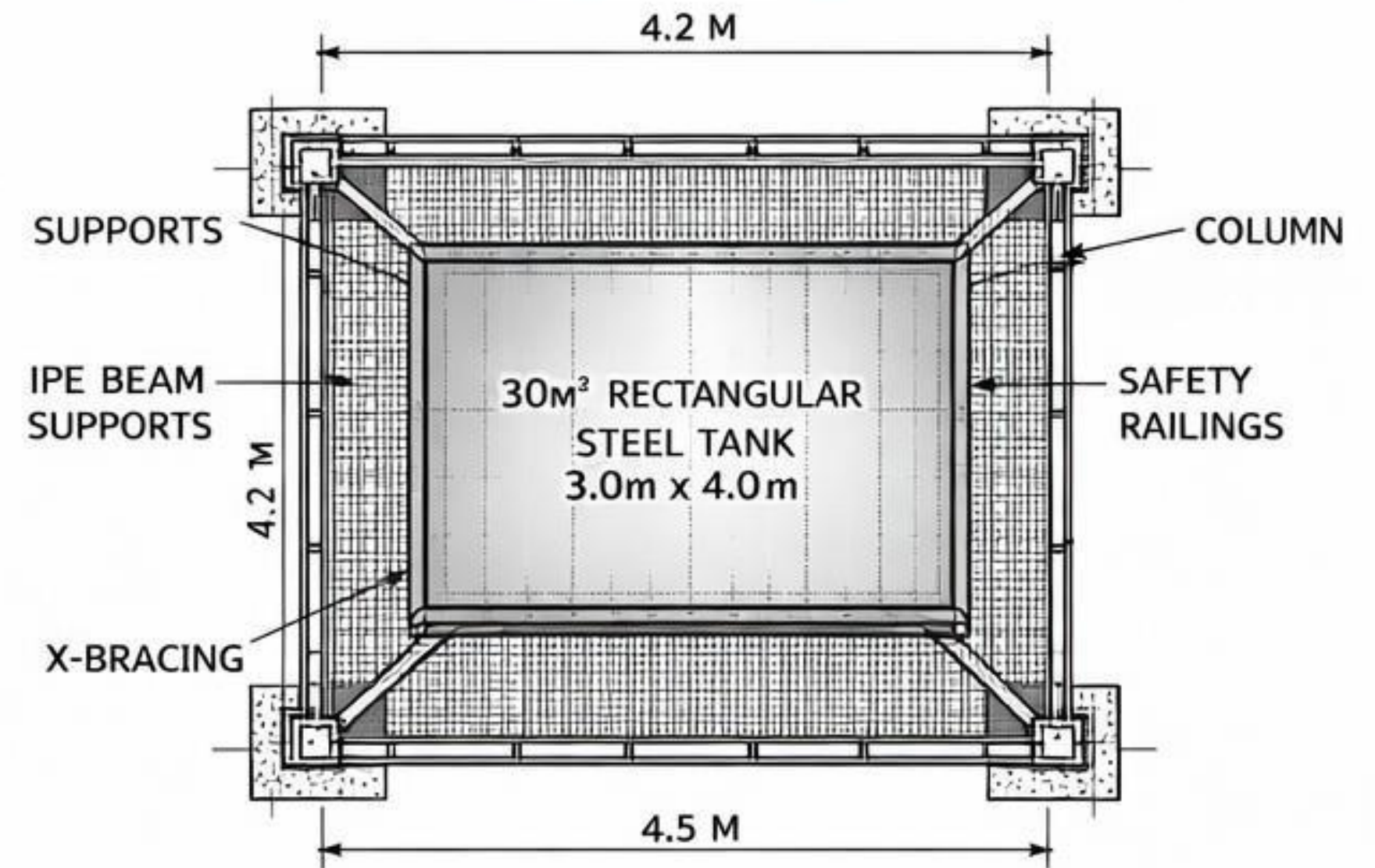
PLAN VIEW
