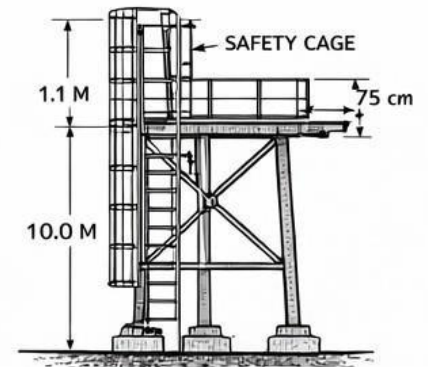
LADDER SECTION
