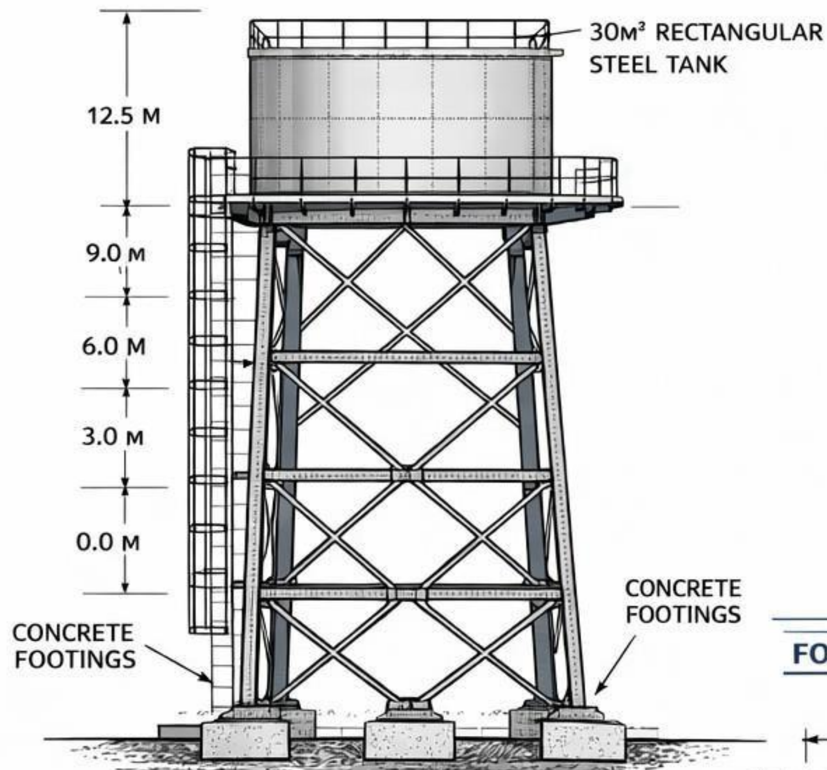
ELEVATION VIEW
