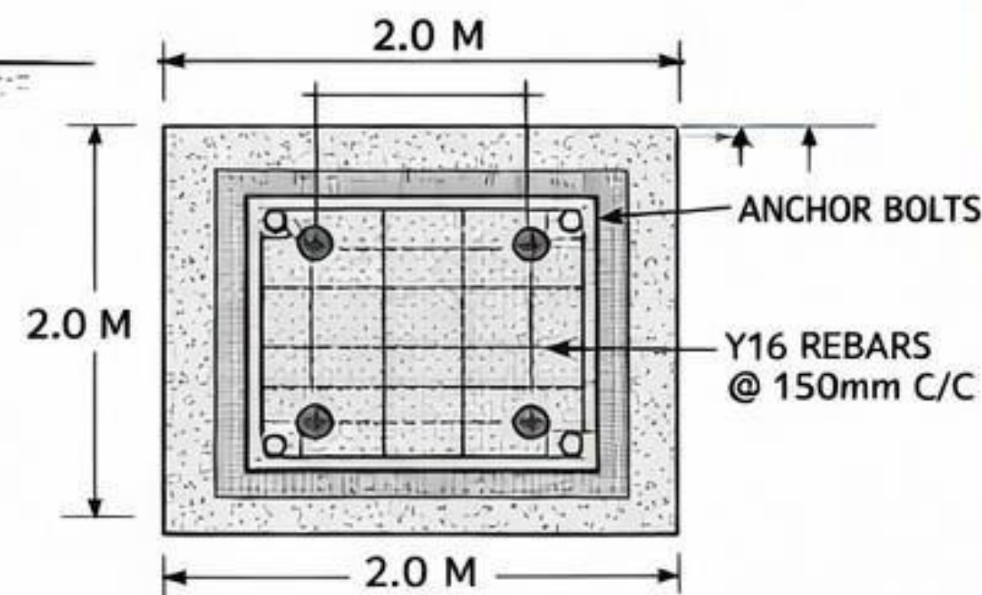
FOUNDATION DETAILS
