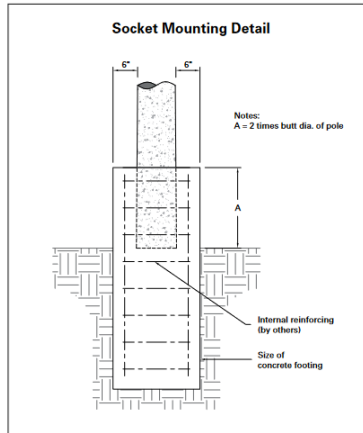
Figure 2: Pole Socket Mounting with Reinforced Concrete
