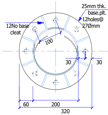
25mm thk. base plate plan detail
