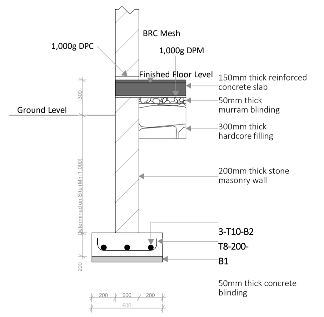
Strip Footing Section
