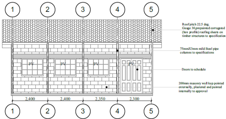
ELEVATION 03 SCALE 1:100
