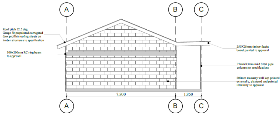
ELEVATION 04 SCALE 1:100
