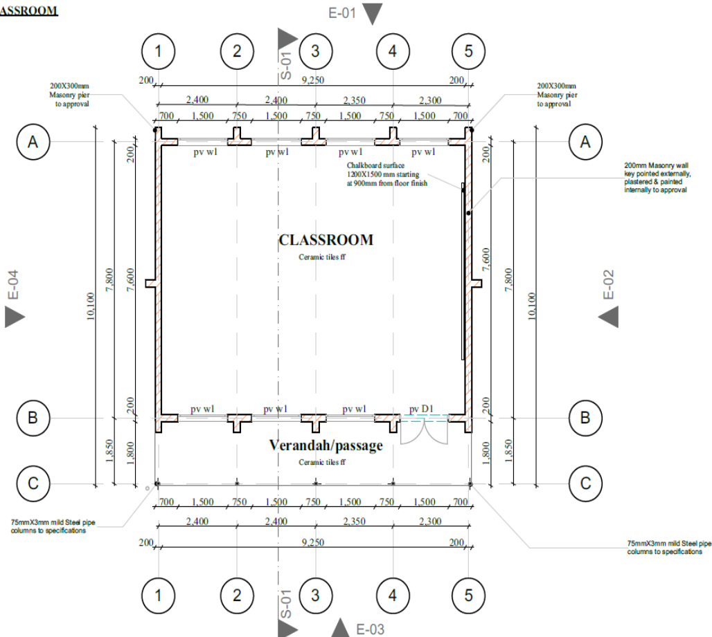
FLOOR PLAN LAYOUT
