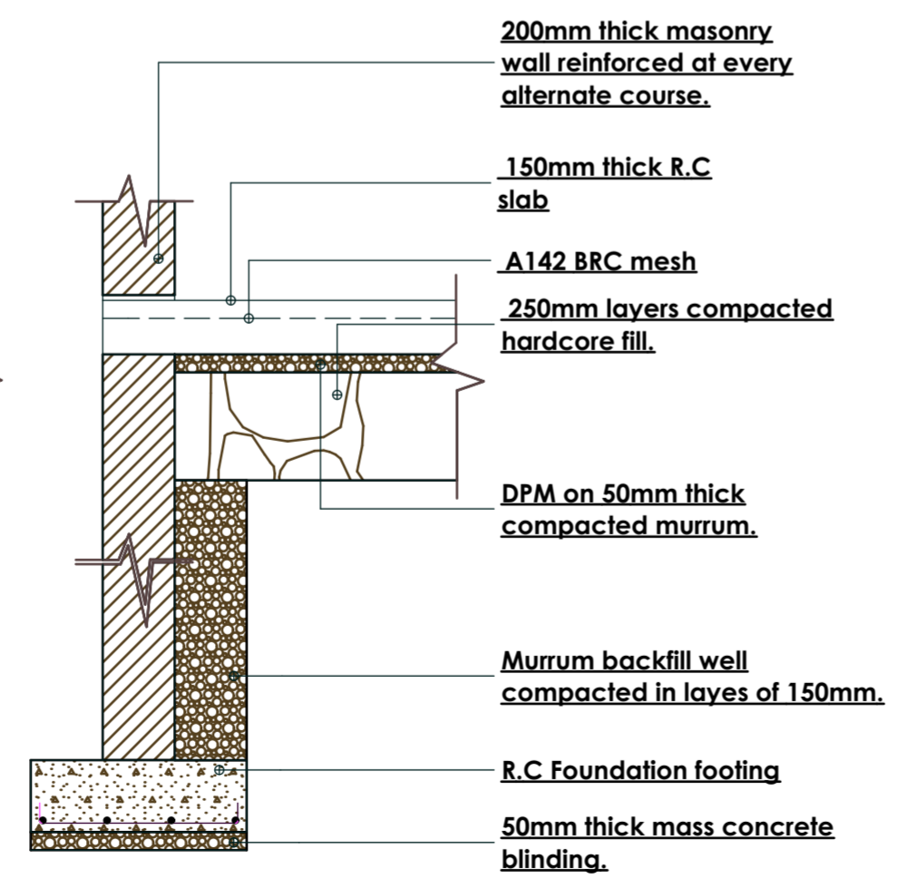
TYPICAL EXTERNAL FOUNDATION WALLS SCALE 1:25
