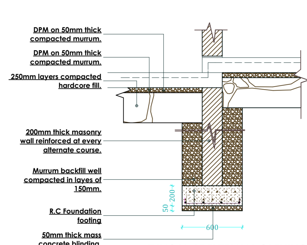
TYPICAL AT EXTERNAL OPENING FOUNDATION WALLS SCALE 1:25
