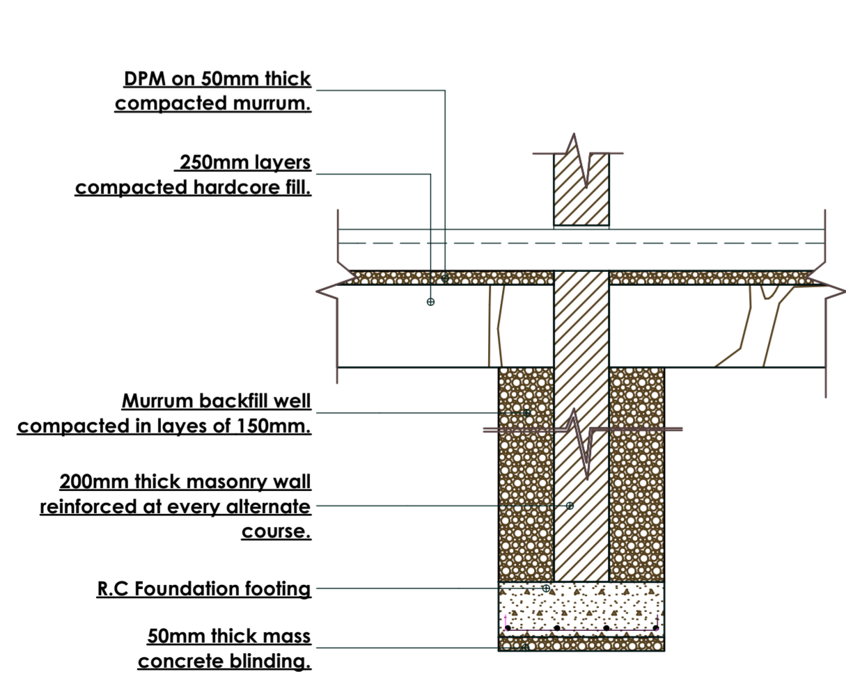
TYPICAL INTERNAL FOUNDATION WALLS SCALE 1:25
