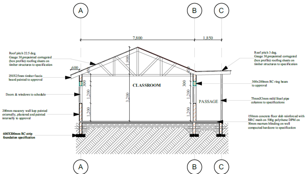
SECTION 01 SCALE 1:100
