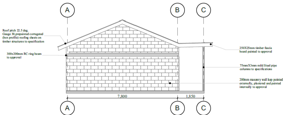
ELEVATION 04 SCALE 1:100
