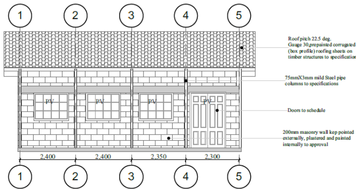
ELEVATION 03 SCALE 1:100
