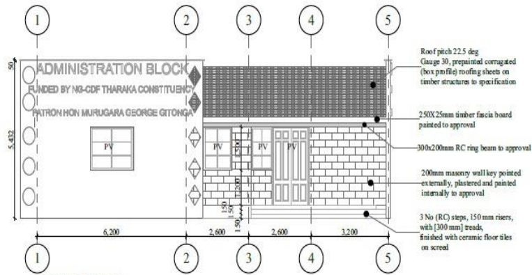
ELEVATION 01 SCALE 1:100
