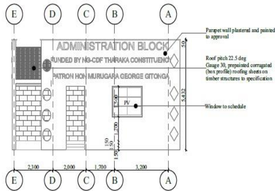
ELEVATION 02 SCALE 1:100
