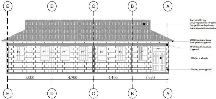
ELEVATION 01 SCALE 1:100
