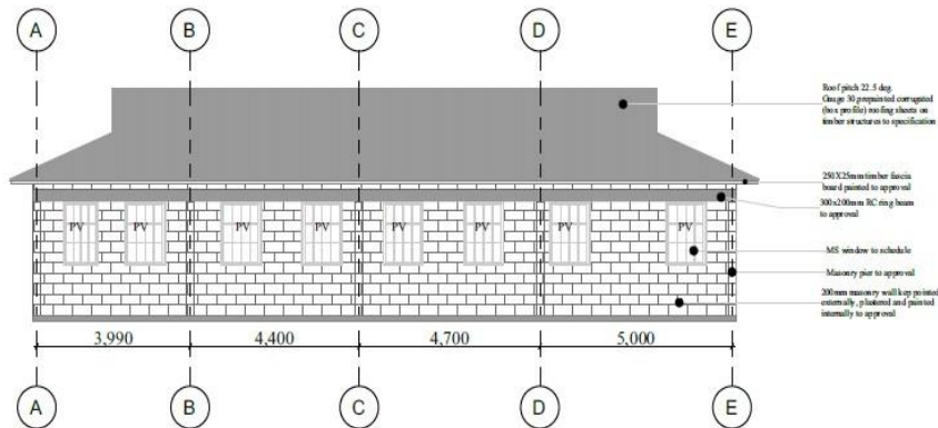
ELEVATION 02 SCALE 1:100
