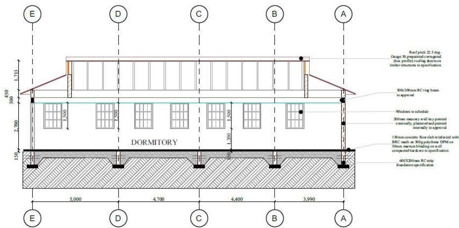
SECTION 01 SCALE 1:100
