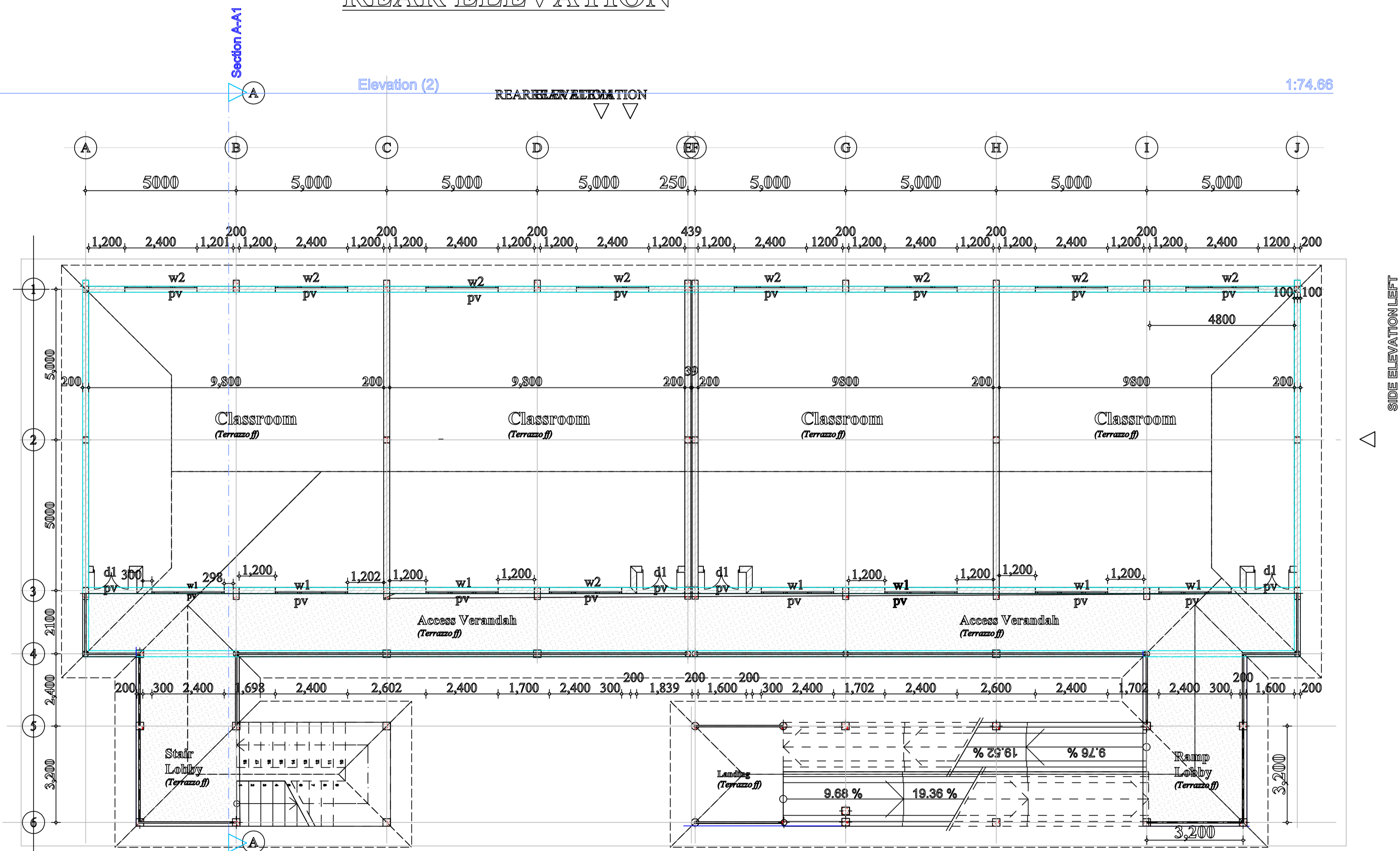
FIRST FLOOR PLAN FRONT ELEVATION
