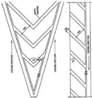
HATCHED AND CHEVRON MARKINGS 1:50
