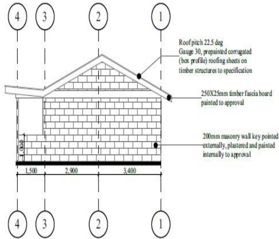
ELEVATION 03 SCALE 1:100
