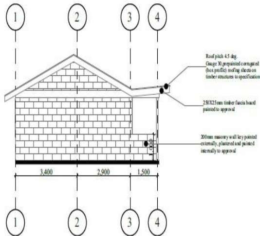
ELEVATION 04 SCALE 1:100
