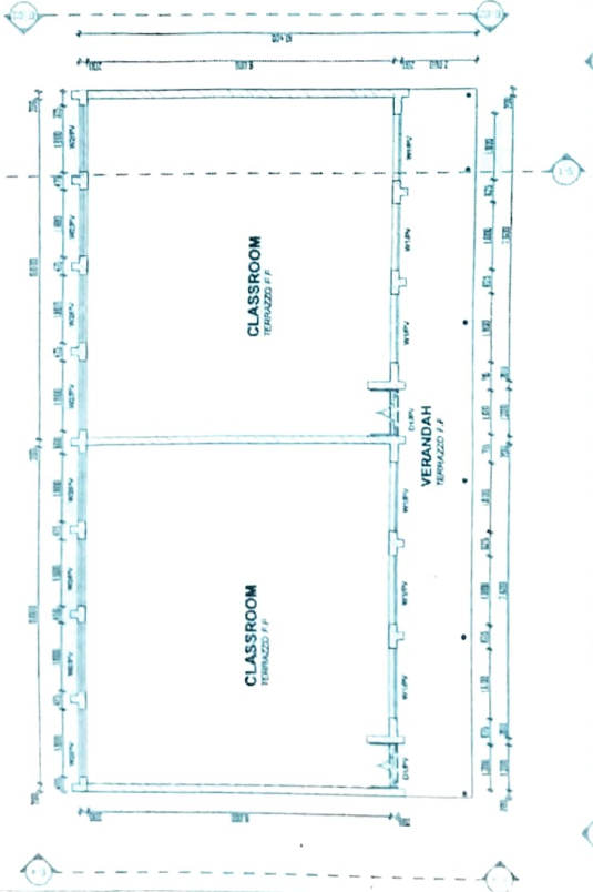
FLOOR PLAN SCALE 1:200
