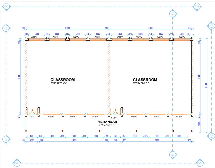
FLOOR PLAN SCALE 1:200
