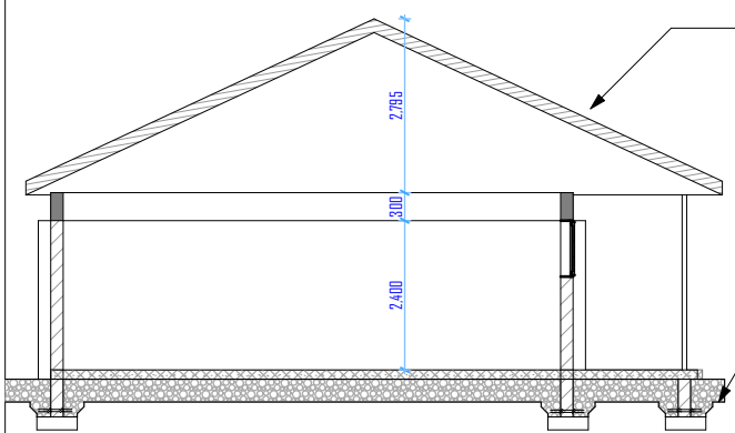
SECTION S-1 SCALE 1:100
