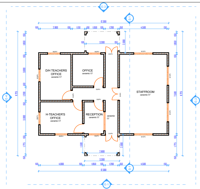
FLOOR PLAN SCALE 1:200
