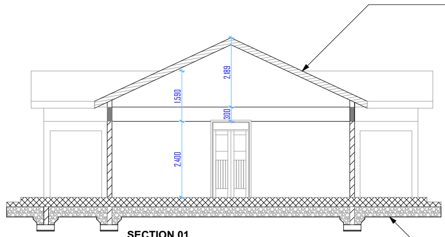
SECTION 01 SCALE 1:200
