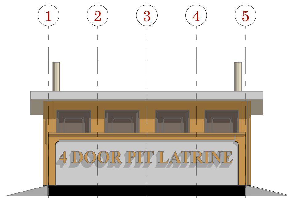
ELEVATION 01 SCALE 1:100
