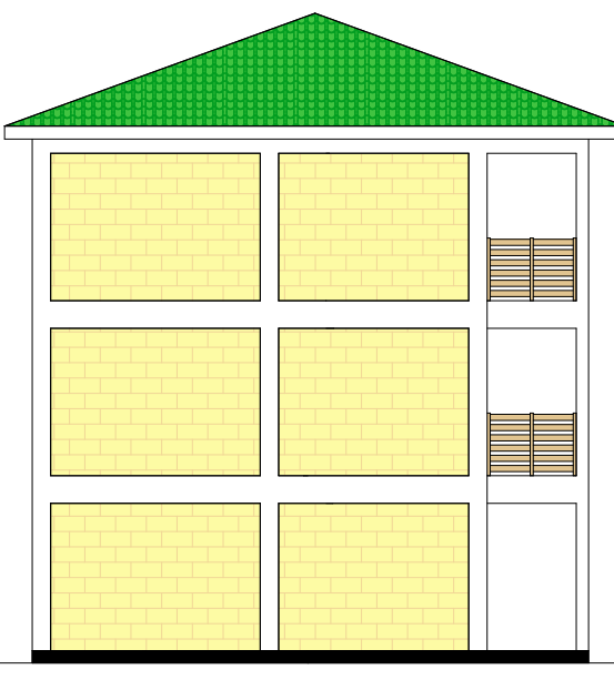
WEST ELEVATION
