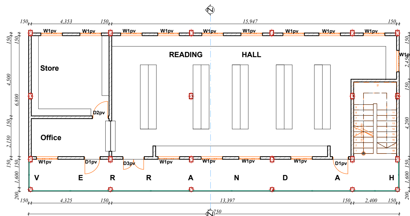
SECOND FLOOR PLAN---LIBRARY
