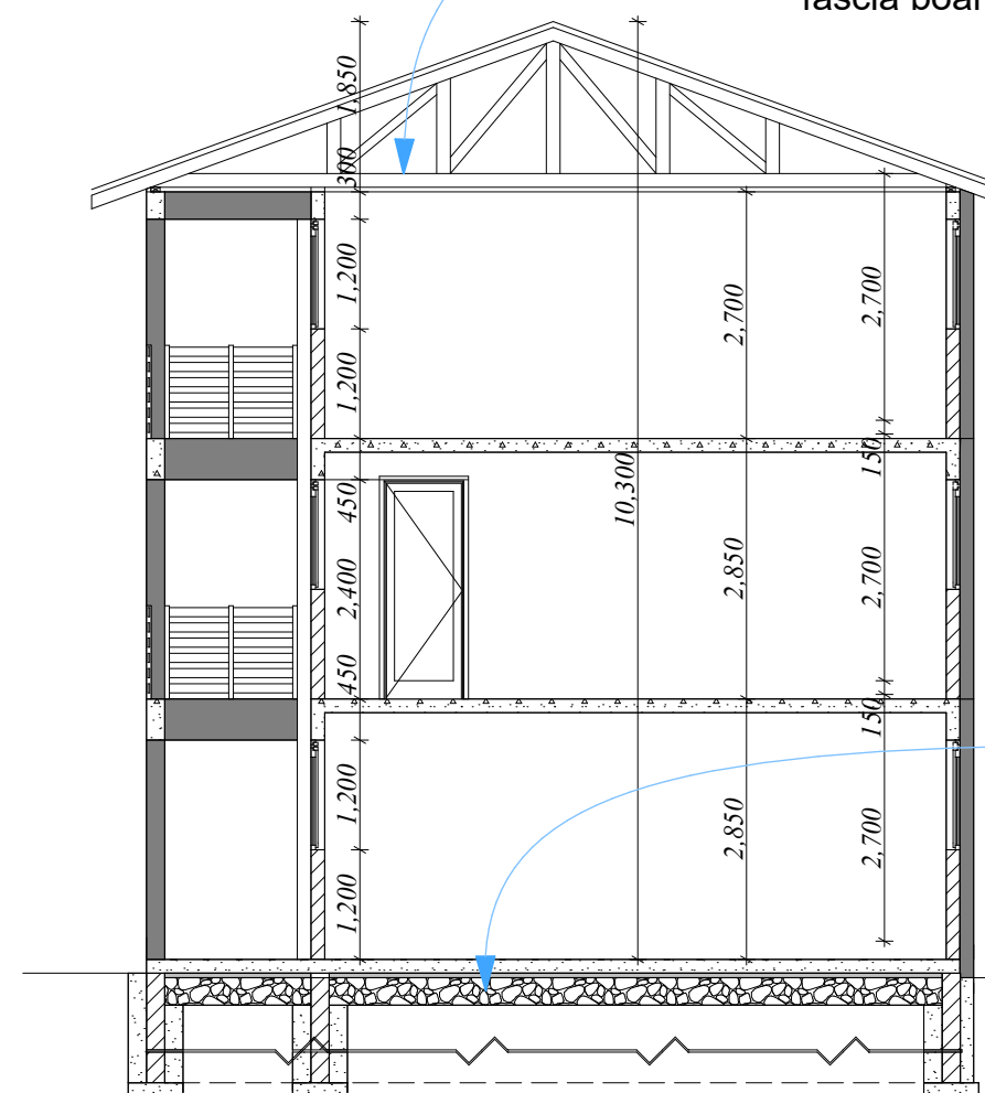
SECTION Z---Z
