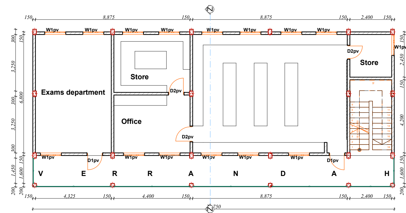
FIRST FLOOR PLAN---COMPUTOR SECTION
