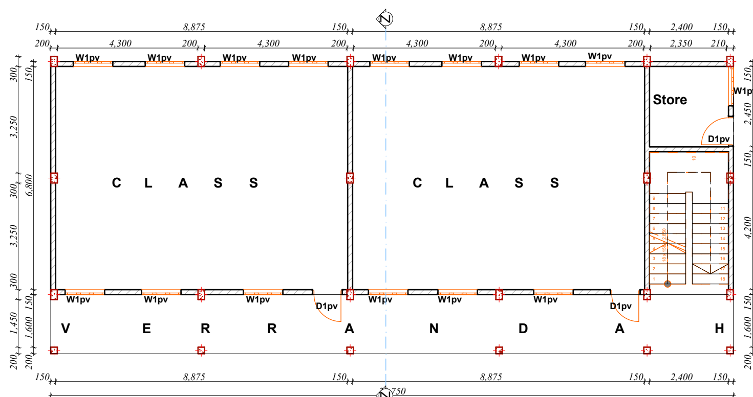
GROUND FLOOR PLAN ---CLASSES
