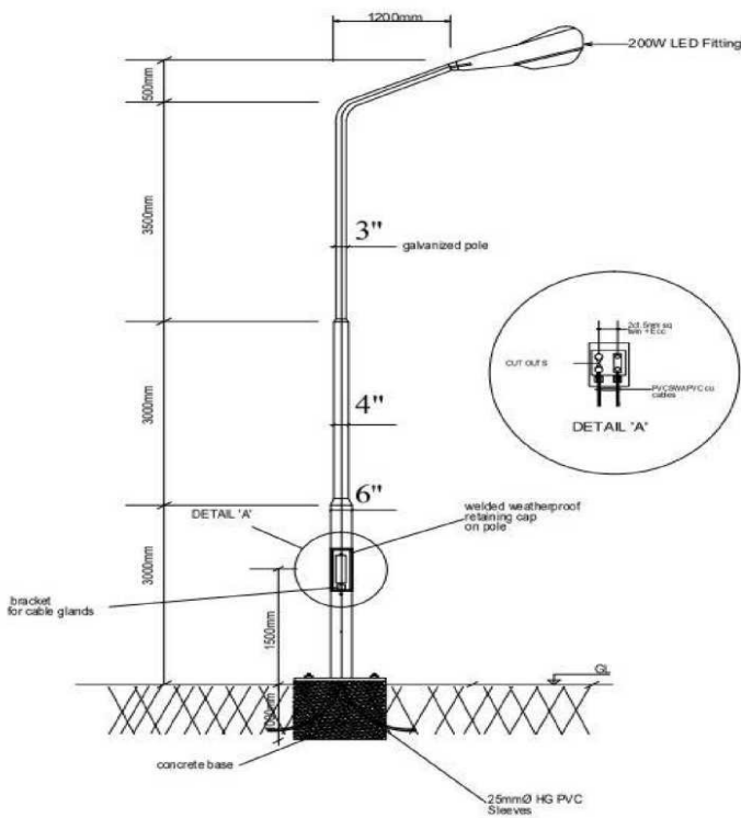
CROSS SECTIONAL DRAWING - SINGLE ARM POLE
