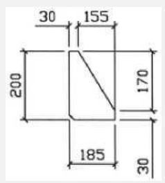
12NQS BASE PLATE STIFFENER—SF1
