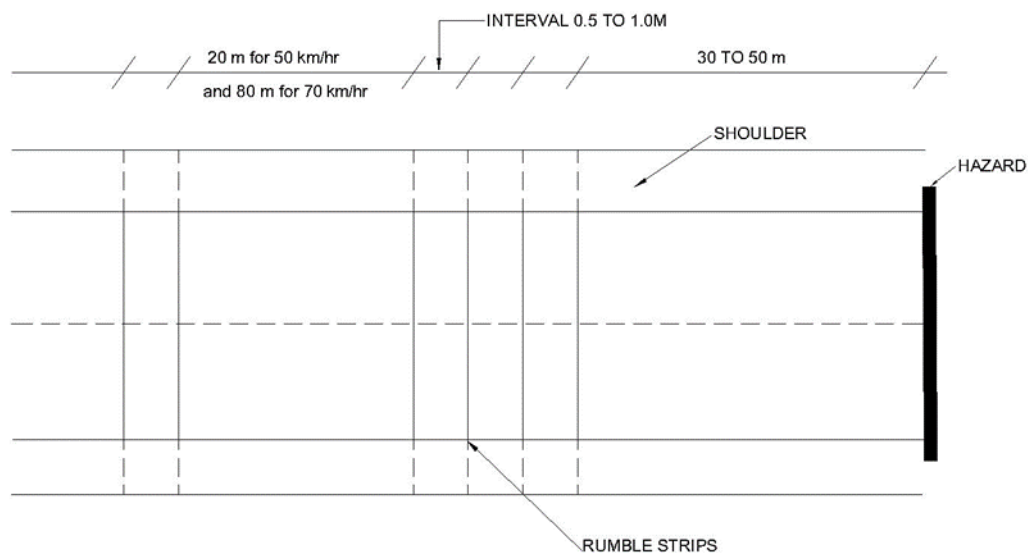
RUMBLE STRIPS DESIGN
