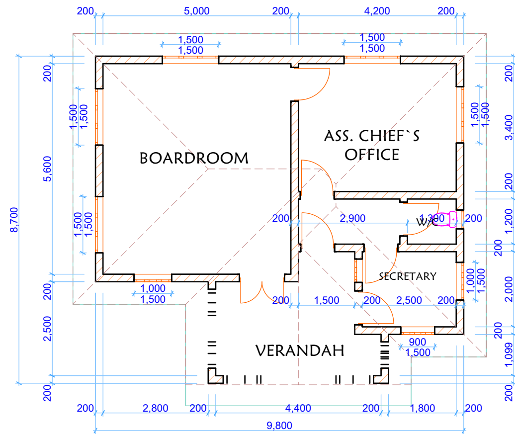
FLOOR PLAN
