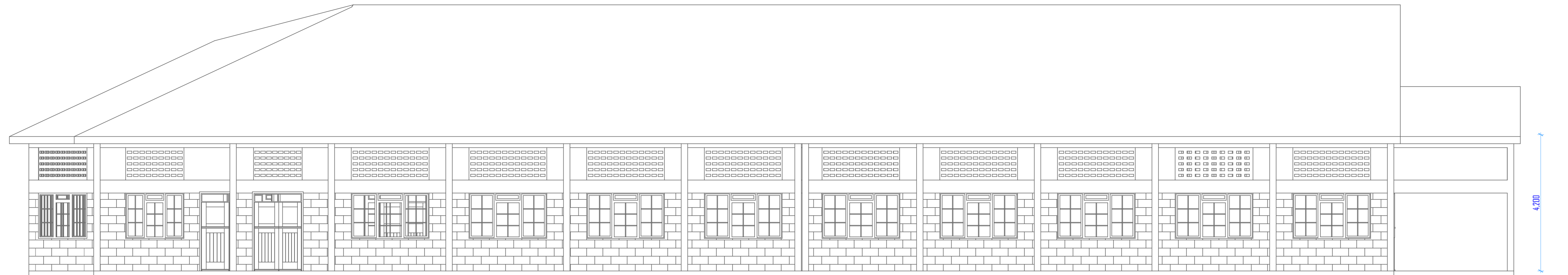
ELEVATION 03 SCALE 1:100
