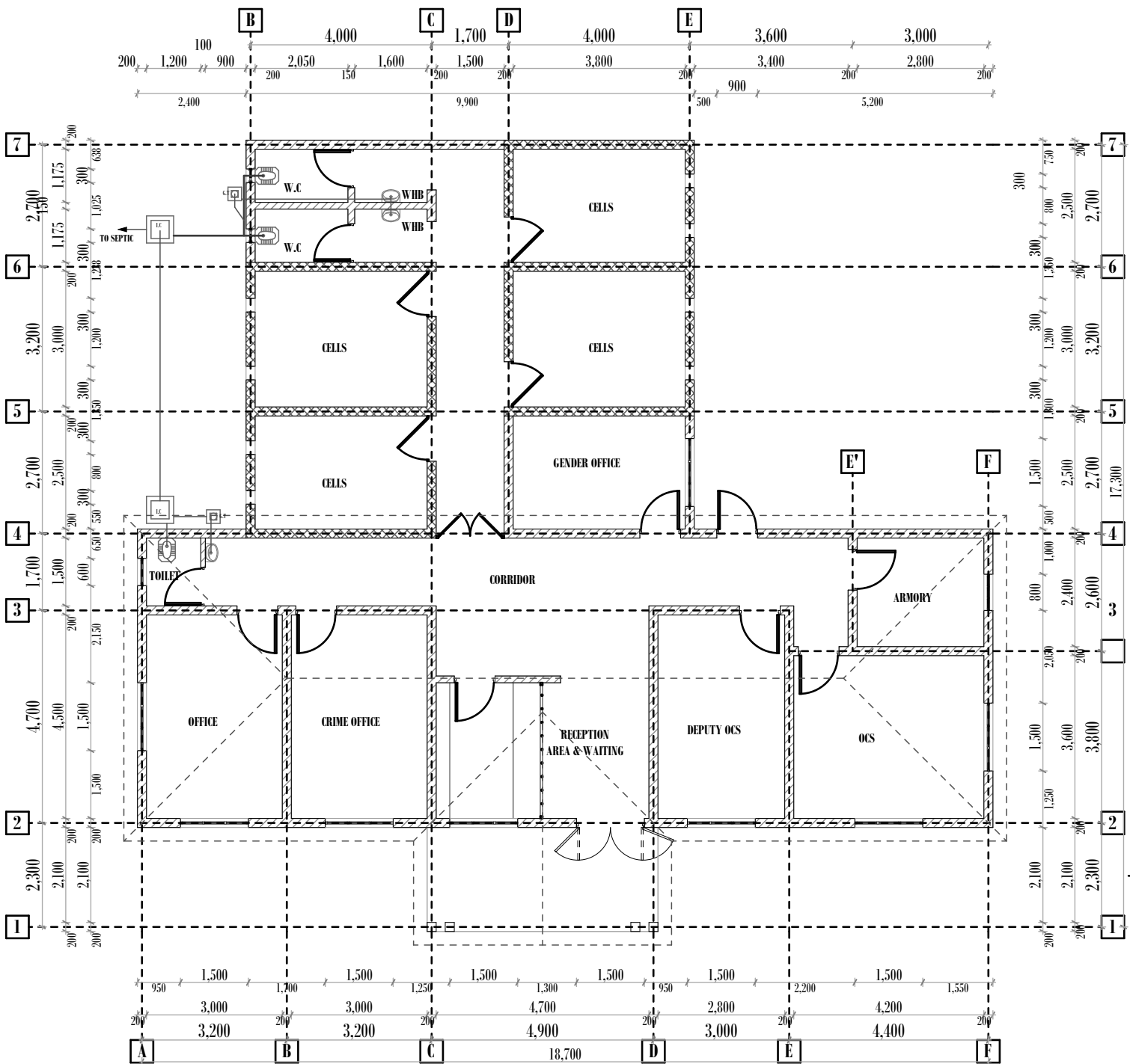
0. Ground Floor (6) 1:125
