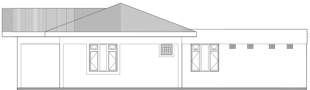
1:100E-02 EAST ELEVATION
