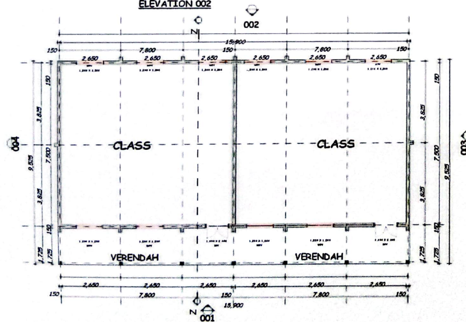
GROUND PLAN
