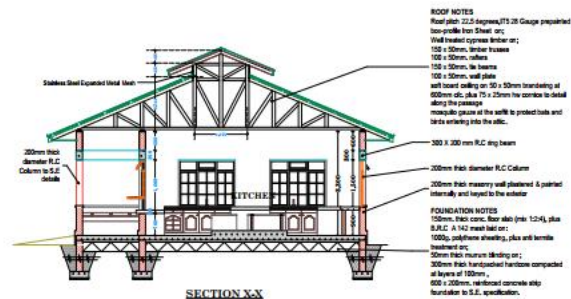
SECTION XX
