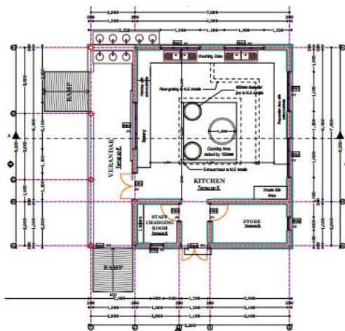
GROUND FLOOR LAYOUT PLAN Scale 1:50
