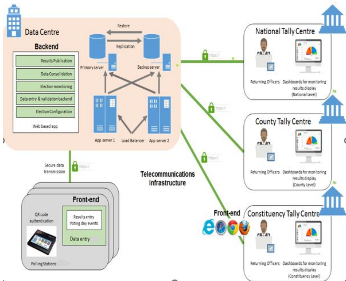
Figure 1 – Current IEMS Network Architecture Layout
