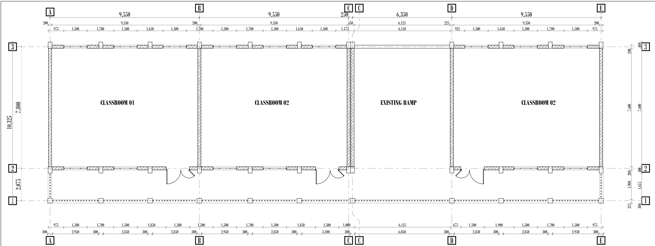
2. SECOND FLOOR 1:150
