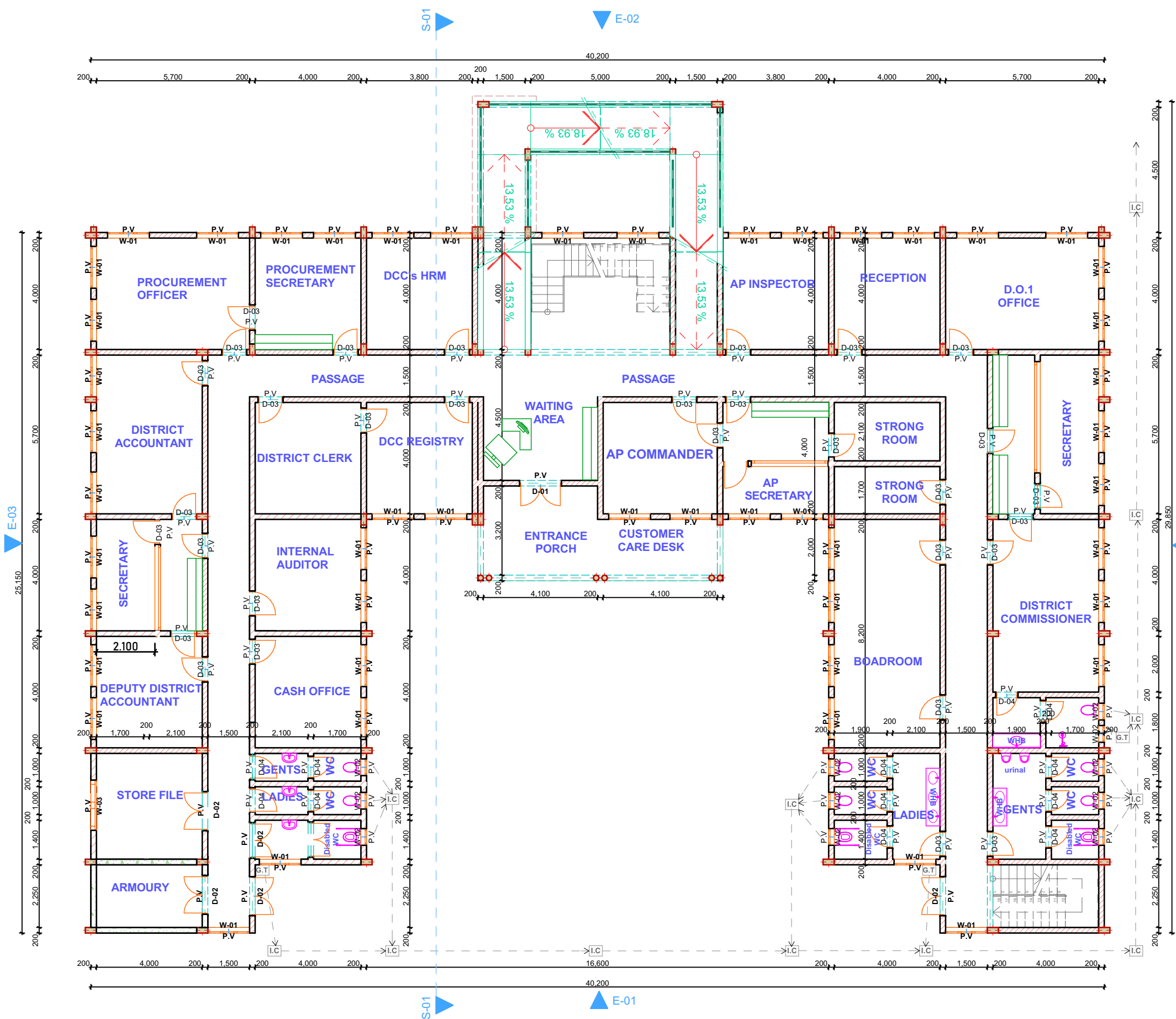
0. Ground Floor Layout Plan 1:150
