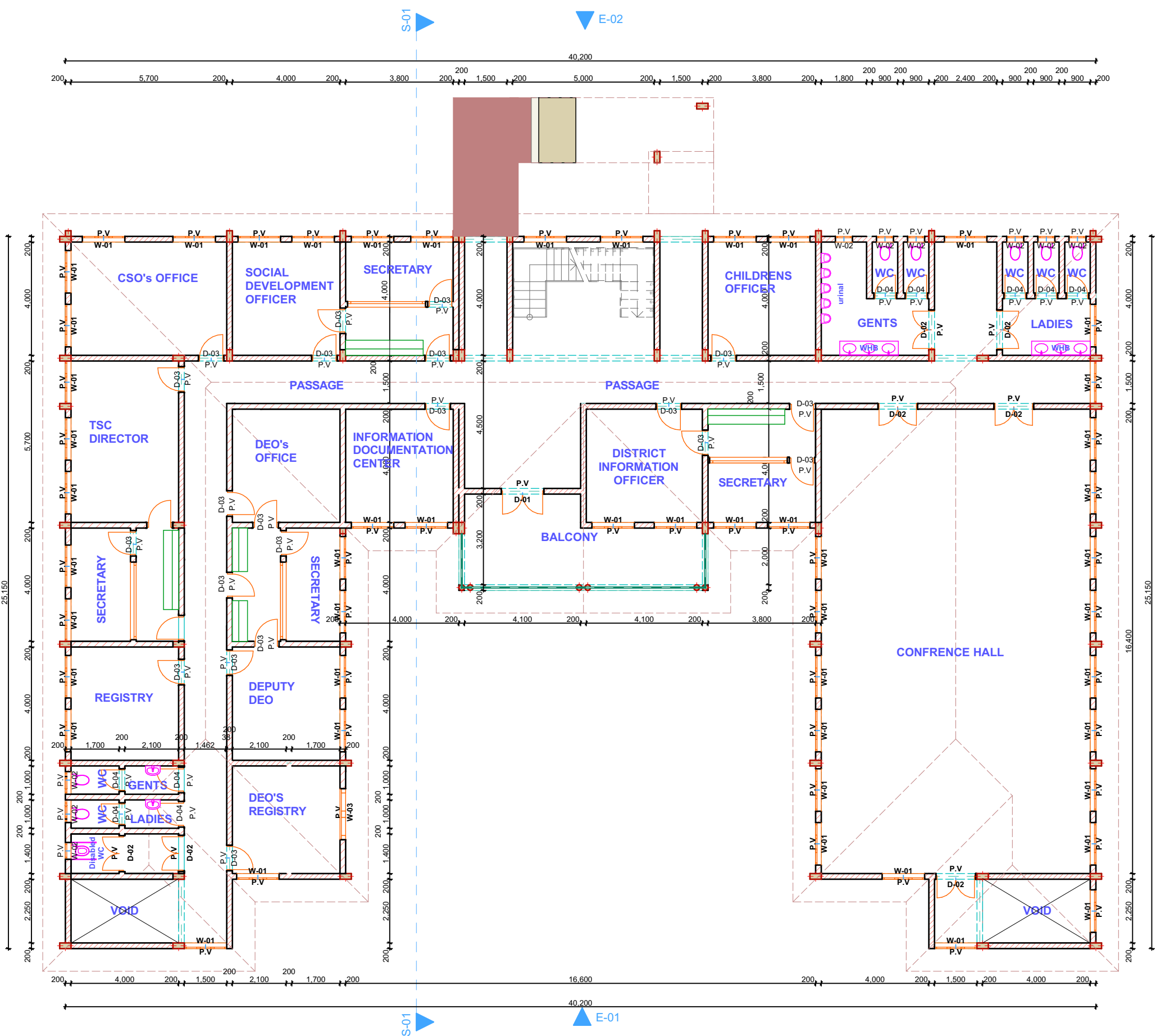
1. First Floor Plan Layout 1:150
