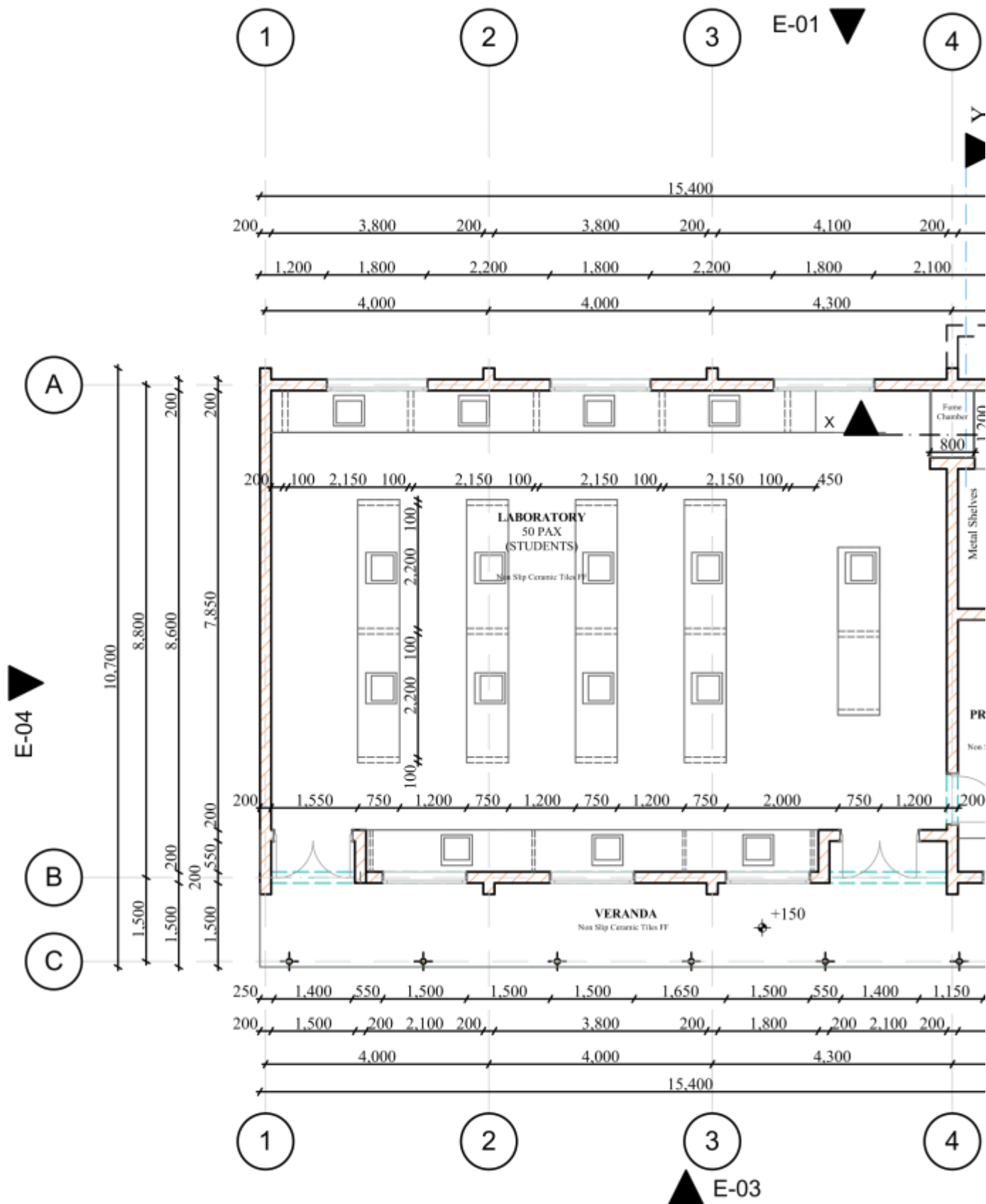
GENERAL LABORATORY FLOOR PLAN 1:100
