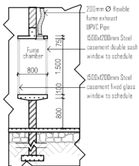
Section X
